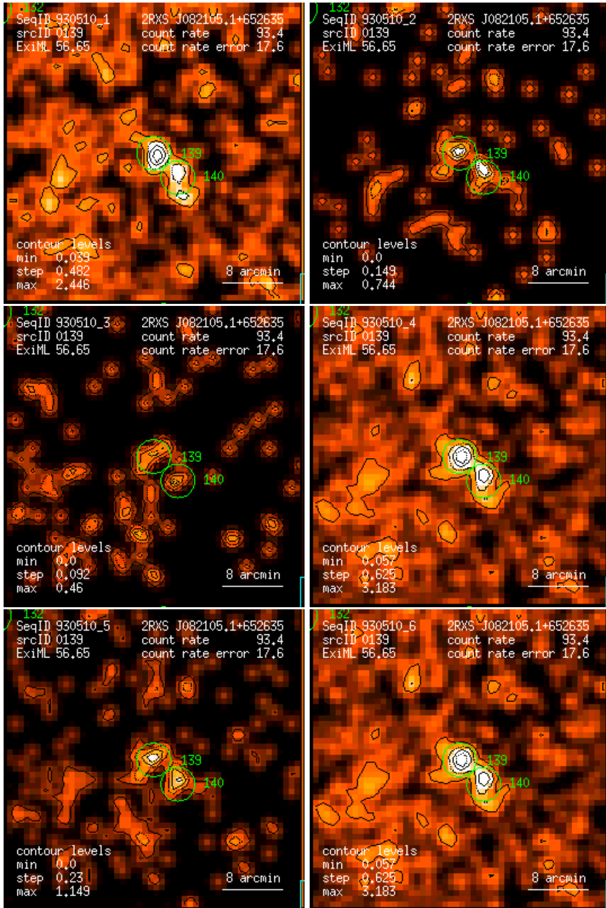
Figure 139: RASS 930510: detection 0139: band rate images, Gaussian filter: (1) PSPC channels 11 – 41, (2) 52 – 90, (3) 91 – 201, (4) 11 – 235, (5) 52 – 201, (6) 11 – 201. Broad band rates in counts/ks. Band rate contour levels in counts/ks/arcmin 2 .
