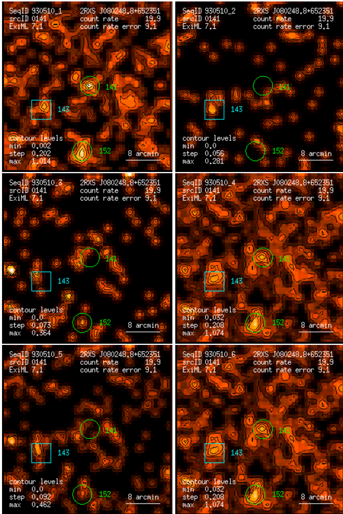
Figure 141: RASS 930510: detection 0141: band rate images, Gaussian filter: (1) PSPC channels 11 – 41, (2) 52 – 90, (3) 91 – 201, (4) 11 – 235, (5) 52 – 201, (6) 11 – 201. Broad band rates in counts/ks. Band rate contour levels in counts/ks/arcmin 2 .
