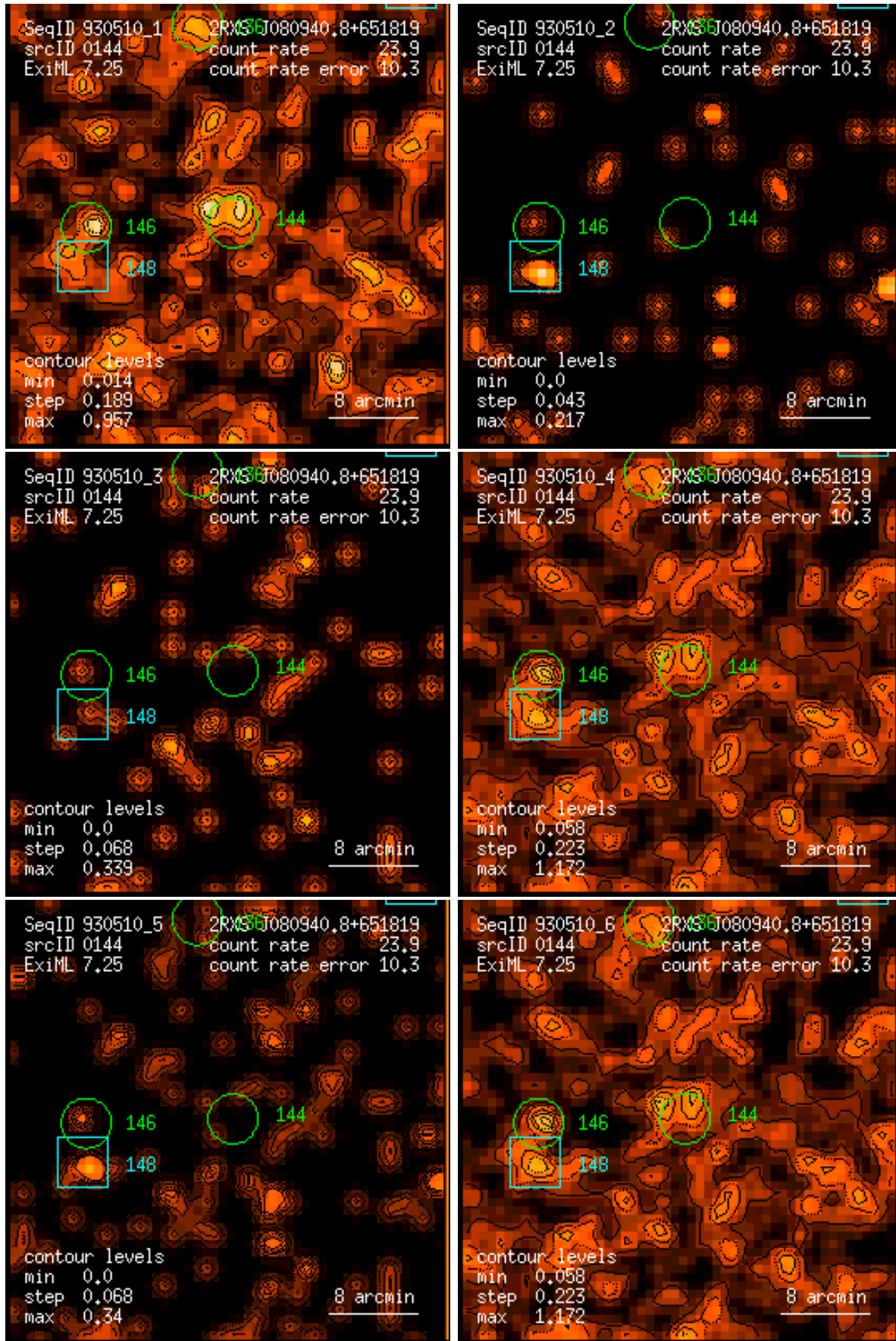
Figure 144: RASS 930510: detection 0144: band rate images, Gaussian filter: (1) PSPC channels 11 – 41, (2) 52 – 90, (3) 91 – 201, (4) 11 – 235, (5) 52 – 201, (6) 11 – 201. Broad band rates in counts/ks. Band rate contour levels in counts/ks/arcmin 2 .
