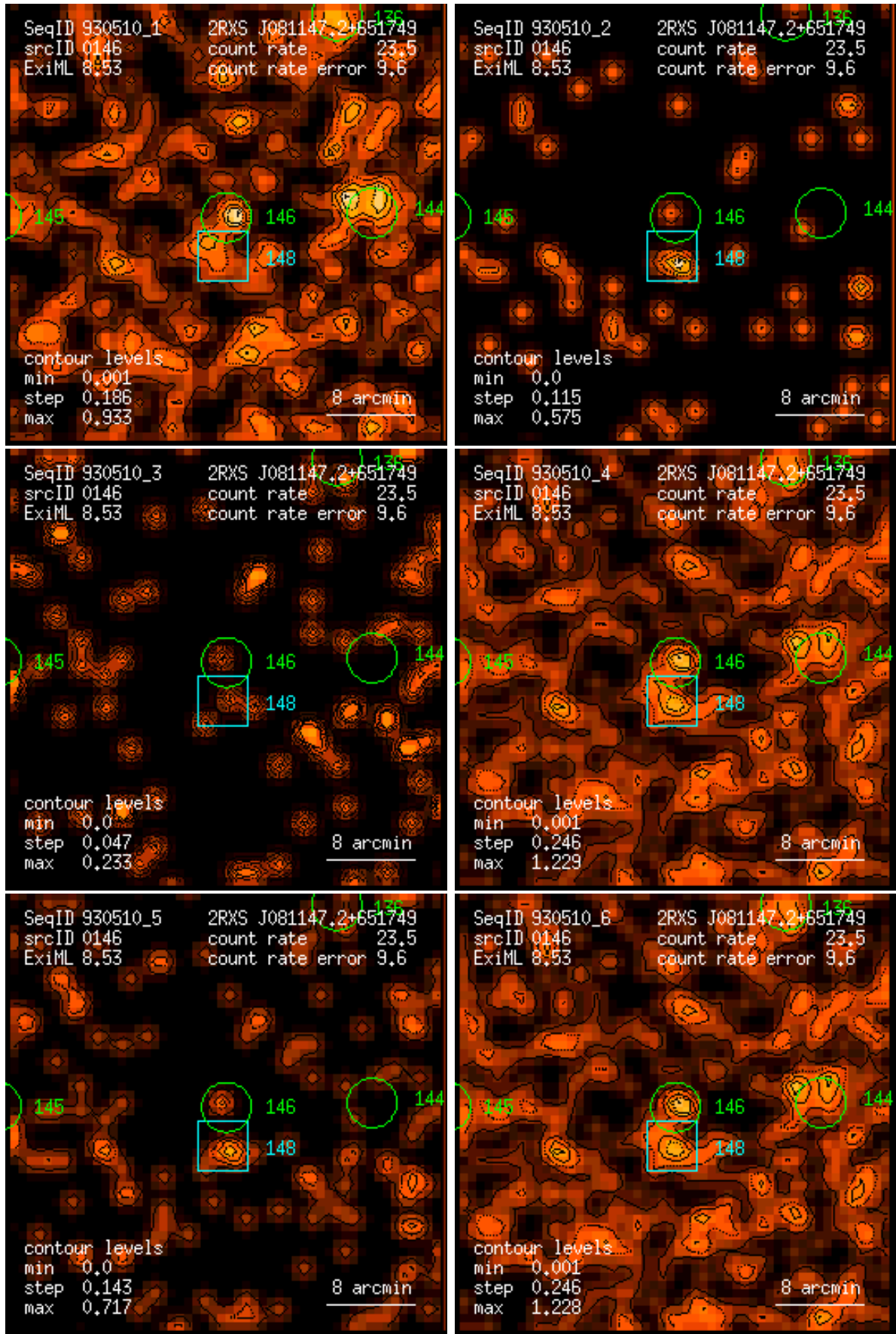
Figure 146: RASS 930510: detection 0146: band rate images, Gaussian filter: (1) PSPC channels 11 – 41, (2) 52 – 90, (3) 91 – 201, (4) 11 – 235, (5) 52 – 201, (6) 11 – 201. Broad band rates in counts/ks. Band rate contour levels in counts/ks/arcmin 2 .
