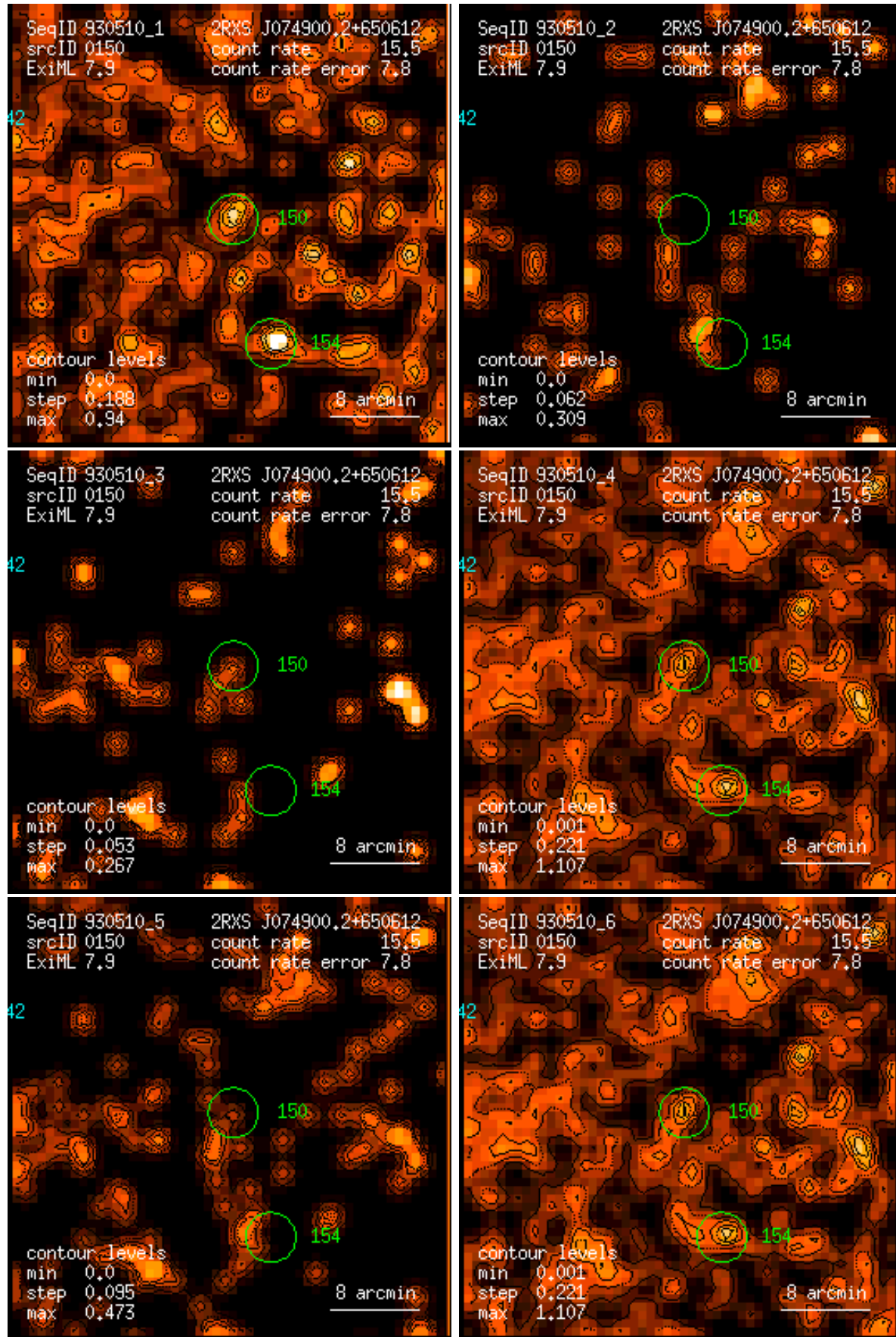
Figure 150: RASS 930510: detection 0150: band rate images, Gaussian filter: (1) PSPC channels 11 – 41, (2) 52 – 90, (3) 91 – 201, (4) 11 – 235, (5) 52 – 201, (6) 11 – 201. Broad band rates in counts/ks. Band rate contour levels in counts/ks/arcmin 2 .
