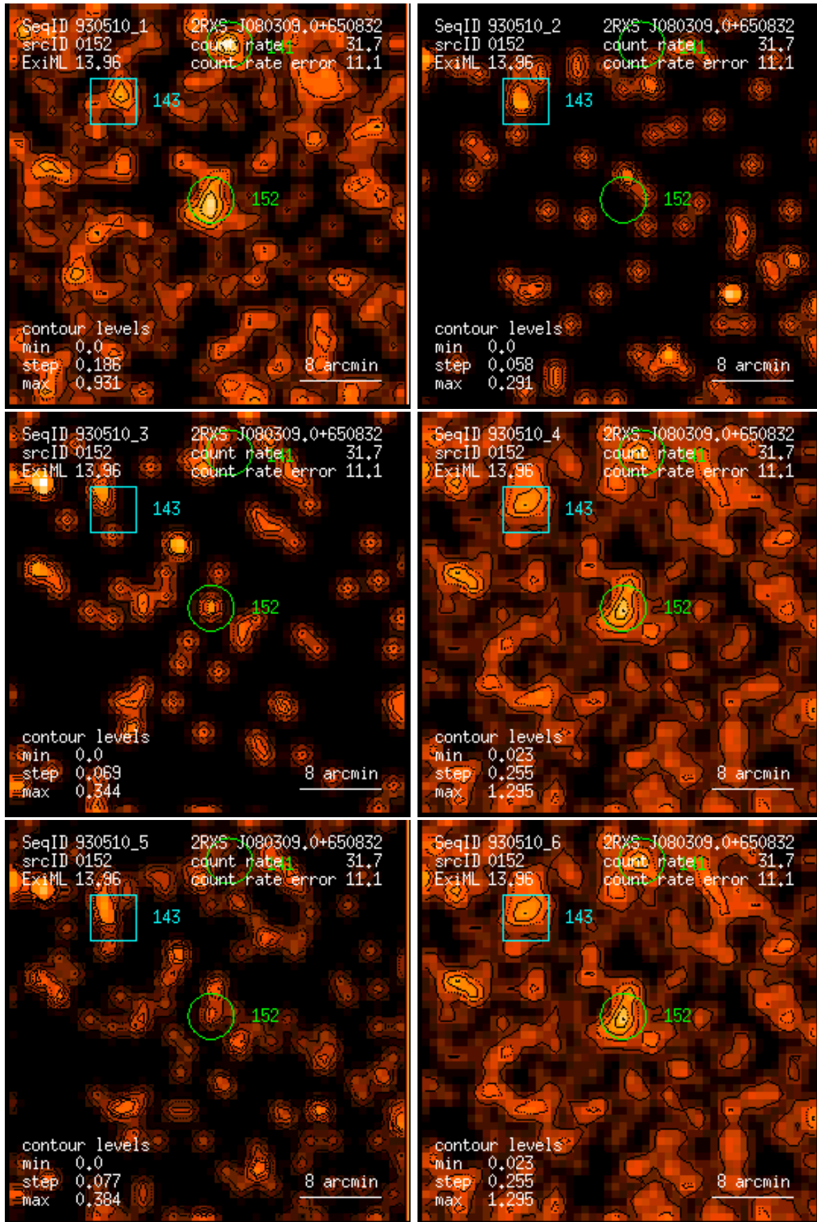
Figure 152: RASS 930510: detection 0152: band rate images, Gaussian filter: (1) PSPC channels 11 – 41, (2) 52 – 90, (3) 91 – 201, (4) 11 – 235, (5) 52 – 201, (6) 11 – 201. Broad band rates in counts/ks. Band rate contour levels in counts/ks/arcmin 2 .
