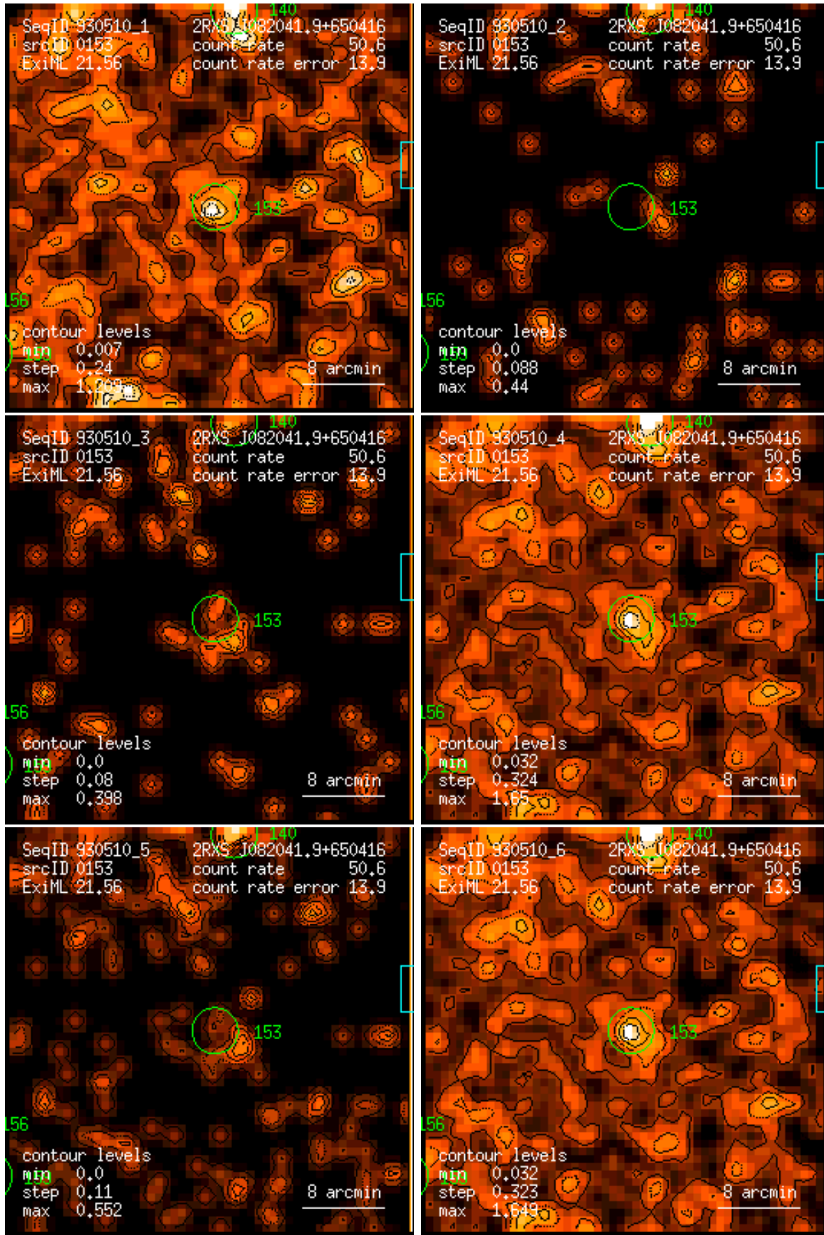
Figure 153: RASS 930510: detection 0153: band rate images, Gaussian filter: (1) PSPC channels 11 – 41, (2) 52 – 90, (3) 91 – 201, (4) 11 – 235, (5) 52 – 201, (6) 11 – 201. Broad band rates in counts/ks. Band rate contour levels in counts/ks/arcmin 2 .
