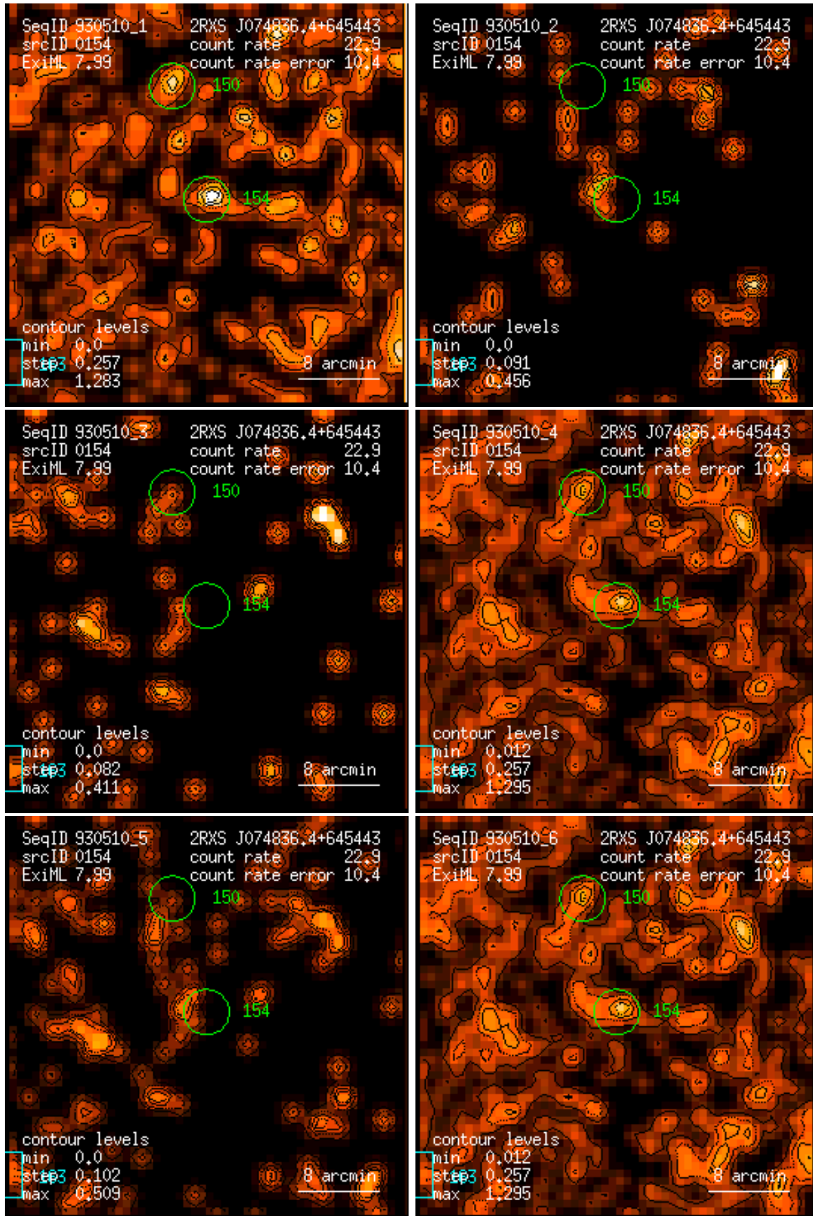
Figure 154: RASS 930510: detection 0154: band rate images, Gaussian filter: (1) PSPC channels 11 – 41, (2) 52 – 90, (3) 91 – 201, (4) 11 – 235, (5) 52 – 201, (6) 11 – 201. Broad band rates in counts/ks. Band rate contour levels in counts/ks/arcmin 2 .
