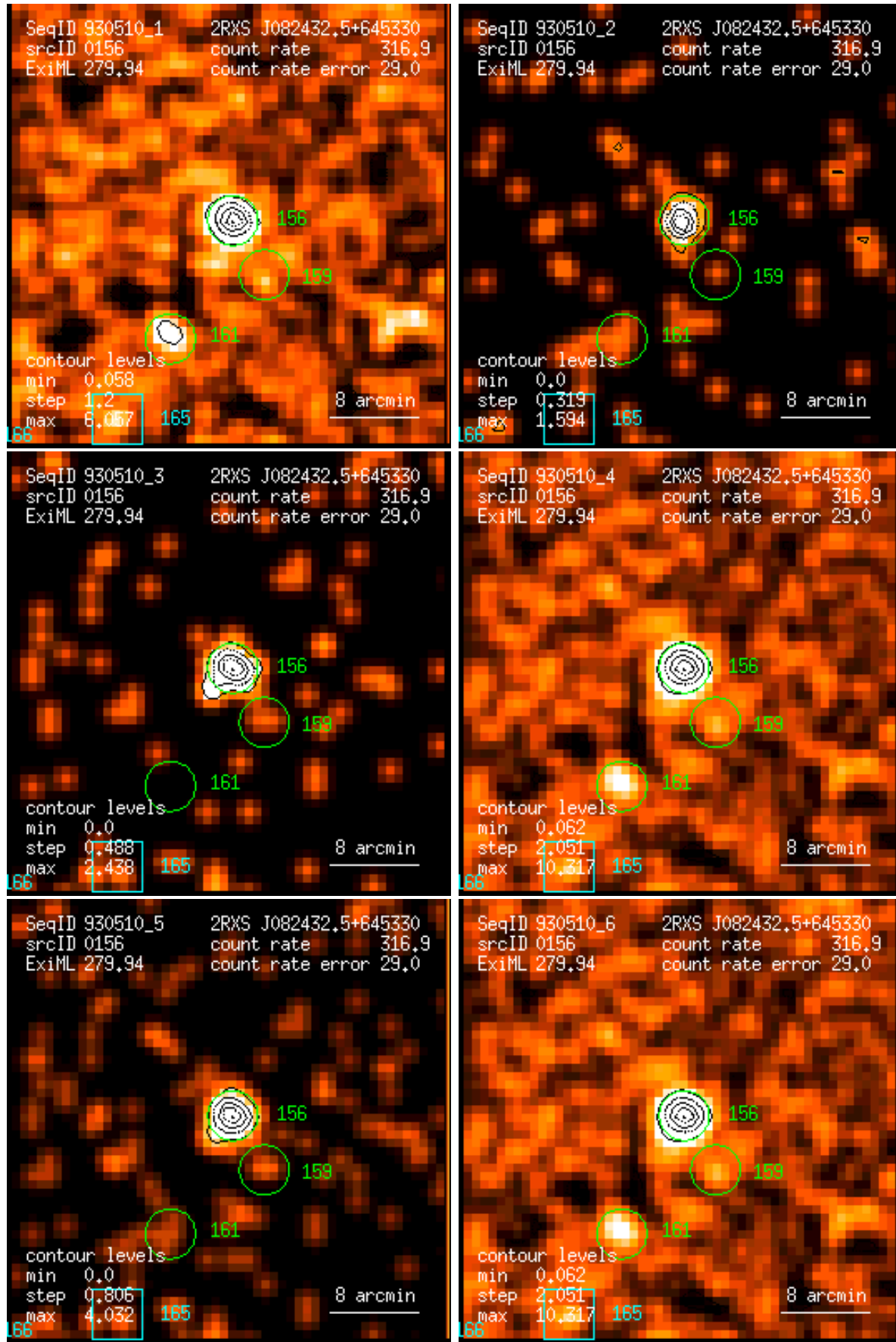
Figure 156: RASS 930510: detection 0156: band rate images, Gaussian filter: (1) PSPC channels 11 – 41, (2) 52 – 90, (3) 91 – 201, (4) 11 – 235, (5) 52 – 201, (6) 11 – 201. Broad band rates in counts/ks. Band rate contour levels in counts/ks/arcmin 2 .
