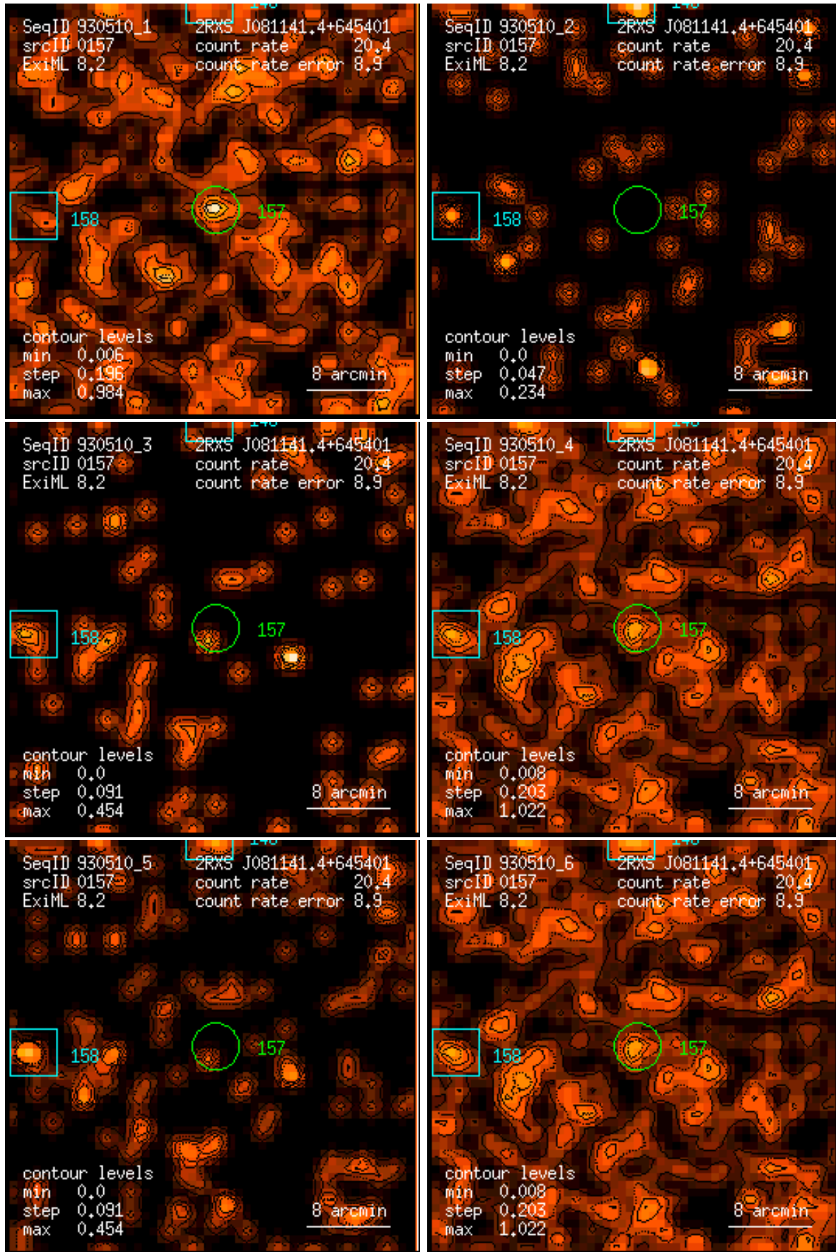
Figure 157: RASS 930510: detection 0157: band rate images, Gaussian filter: (1) PSPC channels 11 – 41, (2) 52 – 90, (3) 91 – 201, (4) 11 – 235, (5) 52 – 201, (6) 11 – 201. Broad band rates in counts/ks. Band rate contour levels in counts/ks/arcmin 2 .
