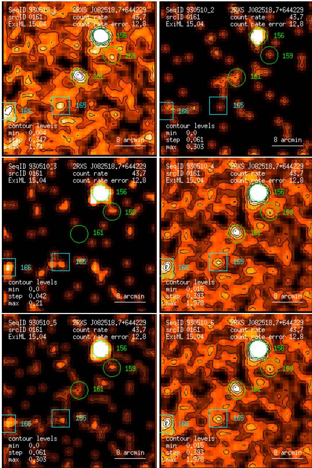
Figure 161: RASS 930510: detection 0161: band rate images, Gaussian filter: (1) PSPC channels 11 – 41, (2) 52 – 90, (3) 91 – 201, (4) 11 – 235, (5) 52 – 201, (6) 11 – 201. Broad band rates in counts/ks. Band rate contour levels in counts/ks/arcmin 2 .
