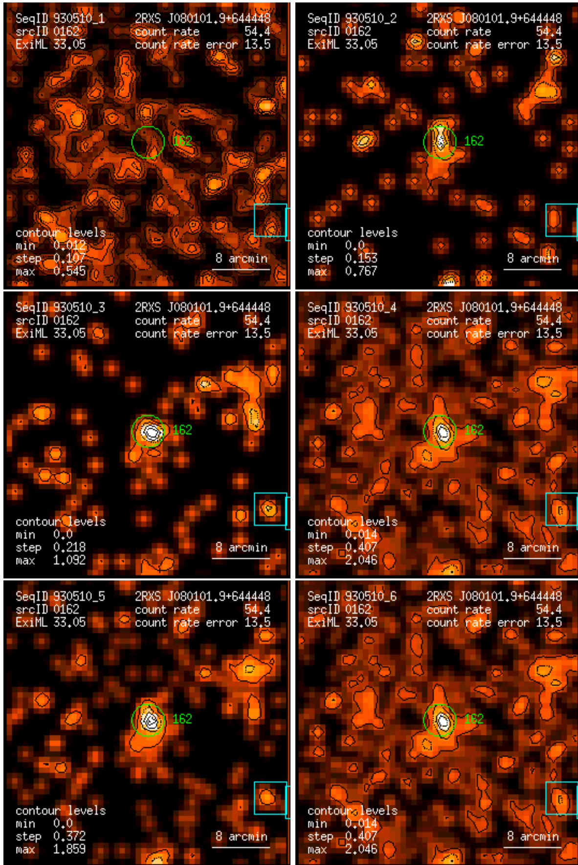
Figure 162: RASS 930510: detection 0162: band rate images, Gaussian filter: (1) PSPC channels 11 – 41, (2) 52 – 90, (3) 91 – 201, (4) 11 – 235, (5) 52 – 201, (6) 11 – 201. Broad band rates in counts/ks. Band rate contour levels in counts/ks/arcmin 2 .
