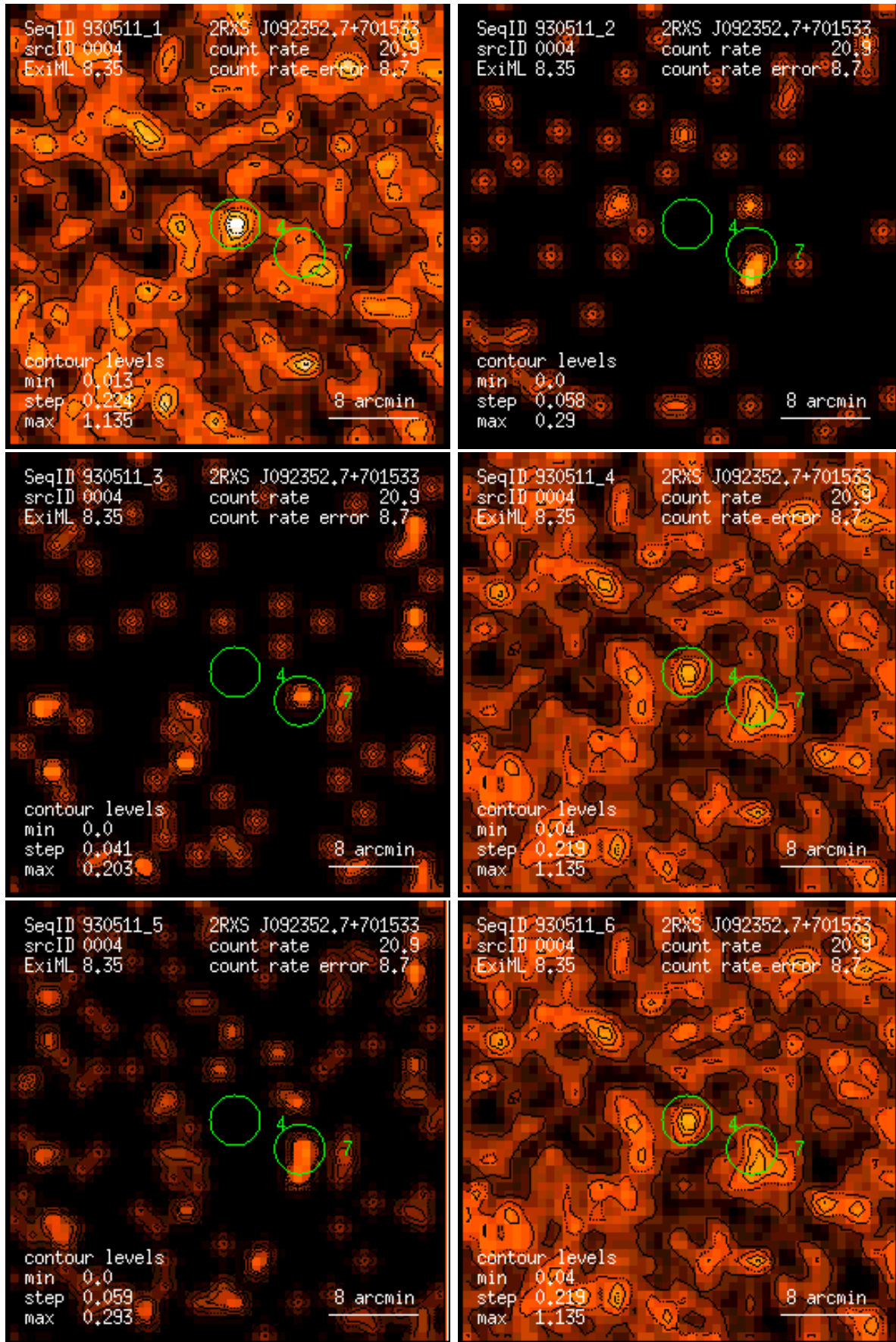
Figure 4: RASS 930511: detection 0004: band rate images, Gaussian filter: (1) PSPC channels 11 – 41, (2) 52 – 90, (3) 91 – 201, (4) 11 – 235, (5) 52 – 201, (6) 11 – 201. Broad band rates in counts/ks. Band rate contour levels in counts/ks/arcmin 2 .
