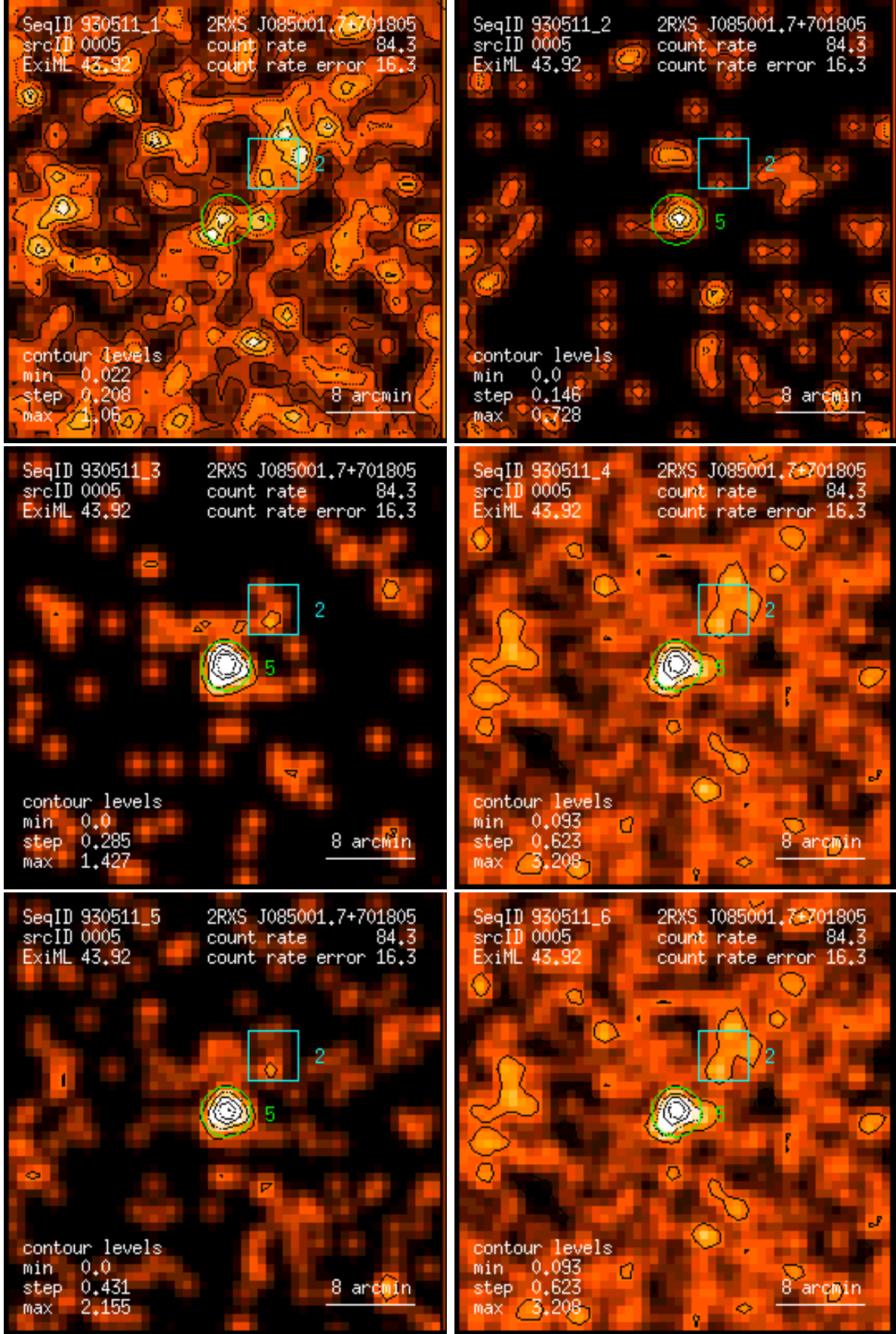
Figure 5: RASS 930511: detection 0005: band rate images, Gaussian filter: (1) PSPC channels 11 – 41, (2) 52 – 90, (3) 91 – 201, (4) 11 – 235, (5) 52 – 201, (6) 11 – 201. Broad band rates in counts/ks. Band rate contour levels in counts/ks/arcmin 2 .
