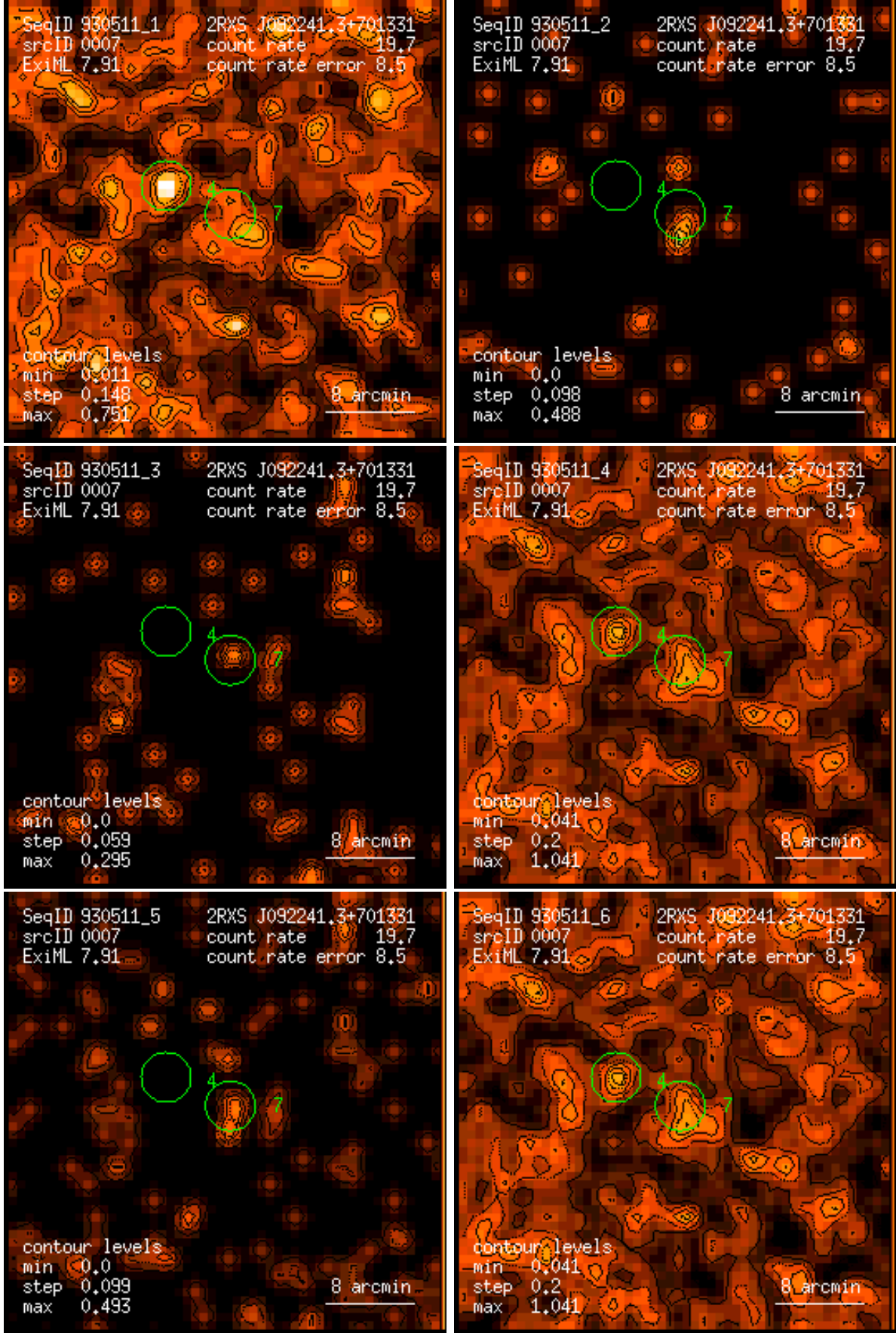
Figure 7: RASS 930511: detection 0007: band rate images, Gaussian filter: (1) PSPC channels 11 – 41, (2) 52 – 90, (3) 91 – 201, (4) 11 – 235, (5) 52 – 201, (6) 11 – 201. Broad band rates in counts/ks. Band rate contour levels in counts/ks/arcmin 2 .
