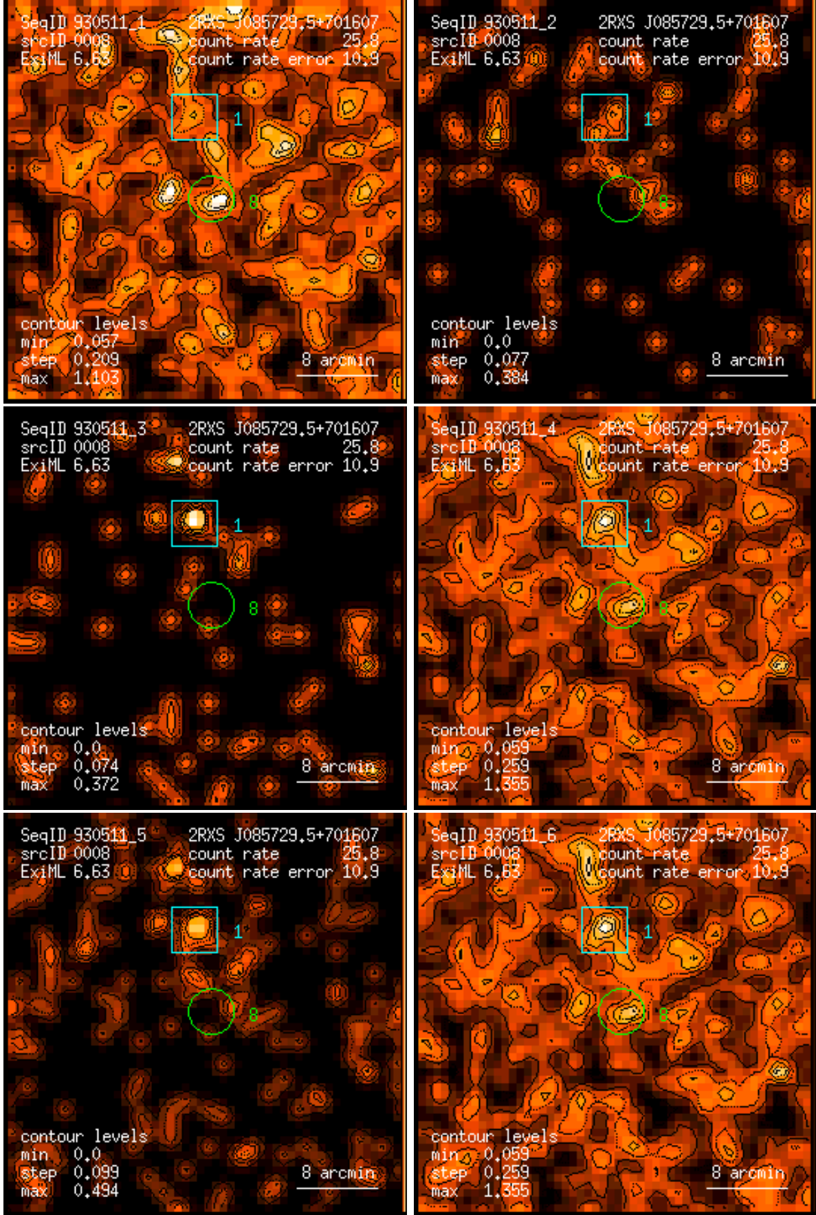
Figure 8: RASS 930511: detection 0008: band rate images, Gaussian filter: (1) PSPC channels 11 – 41, (2) 52 – 90, (3) 91 – 201, (4) 11 – 235, (5) 52 – 201, (6) 11 – 201. Broad band rates in counts/ks. Band rate contour levels in counts/ks/arcmin 2 .
