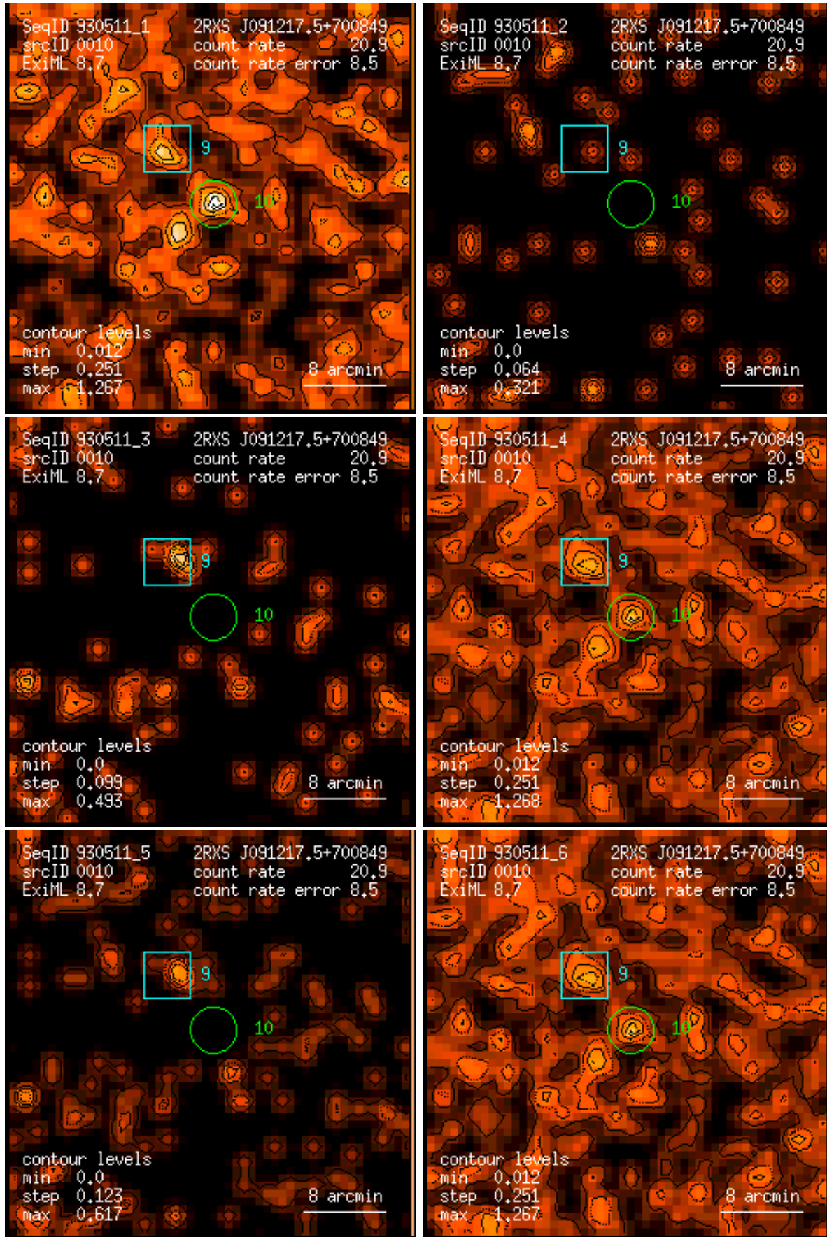
Figure 10: RASS 930511: detection 0010: band rate images, Gaussian filter: (1) PSPC channels 11 – 41, (2) 52 – 90, (3) 91 – 201, (4) 11 – 235, (5) 52 – 201, (6) 11 – 201. Broad band rates in counts/ks. Band rate contour levels in counts/ks/arcmin 2 .
