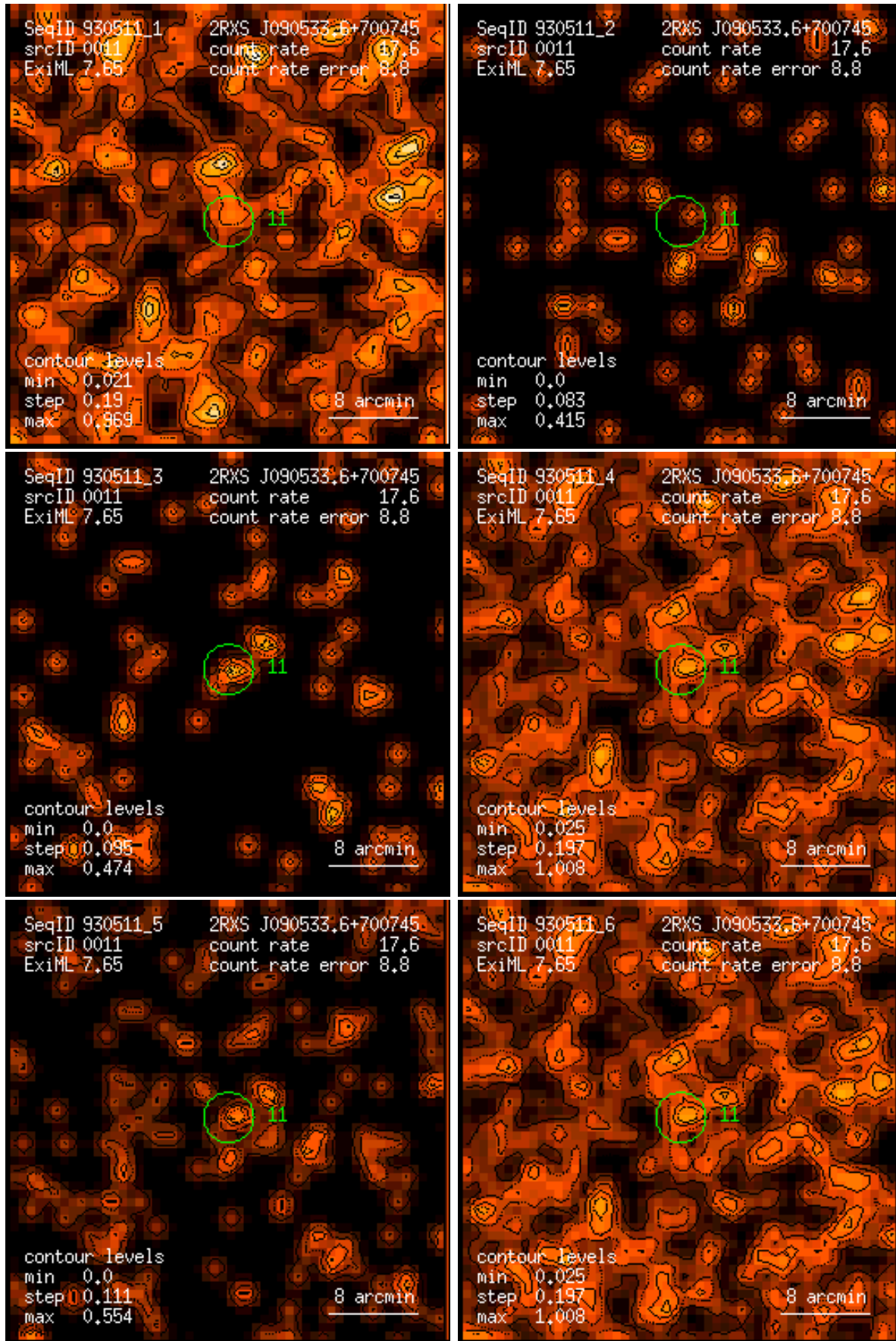
Figure 11: RASS 930511: detection 0011: band rate images, Gaussian filter: (1) PSPC channels 11 – 41, (2) 52 – 90, (3) 91 – 201, (4) 11 – 235, (5) 52 – 201, (6) 11 – 201. Broad band rates in counts/ks. Band rate contour levels in counts/ks/arcmin 2 .
