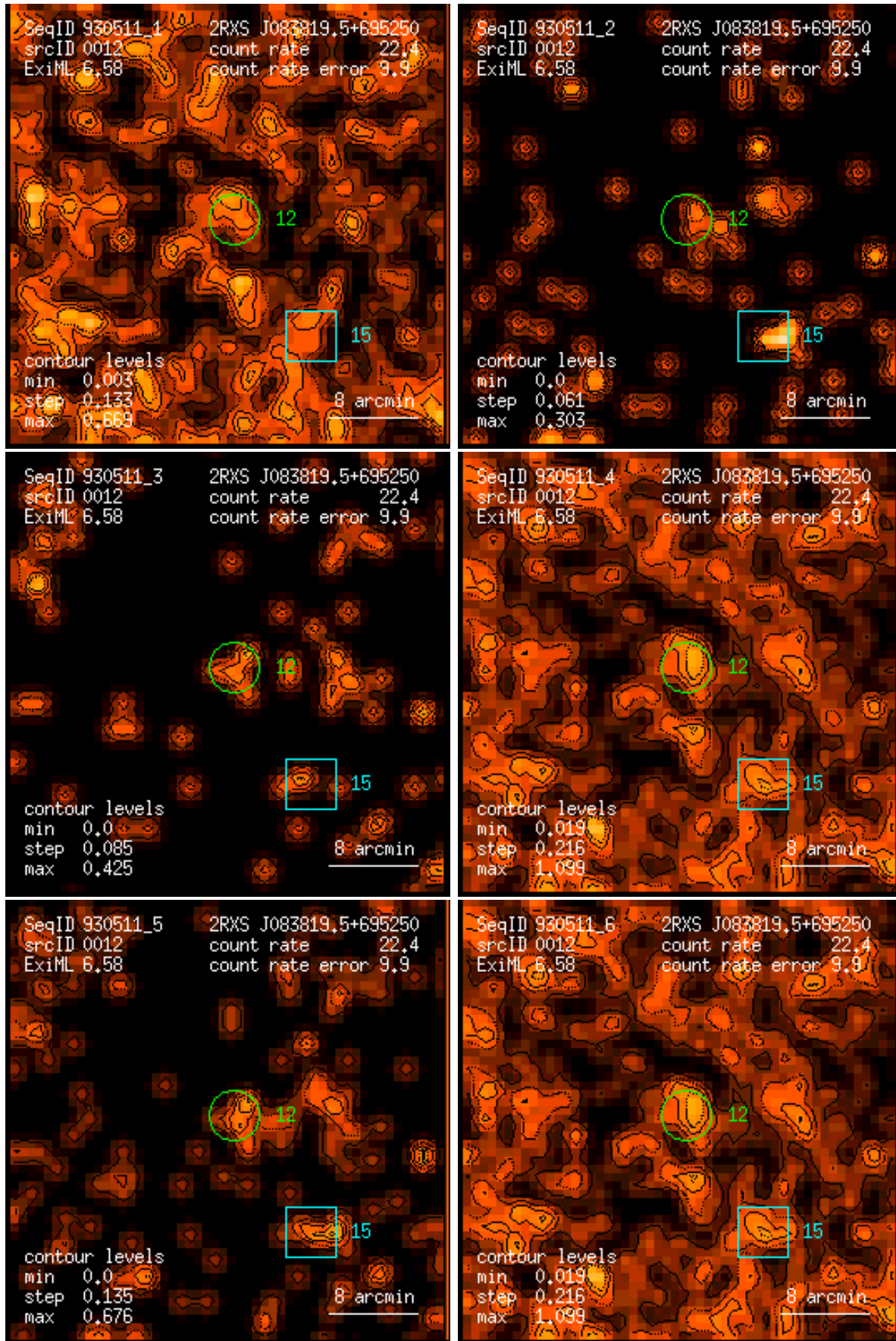
Figure 12: RASS 930511: detection 0012: band rate images, Gaussian filter: (1) PSPC channels 11 – 41, (2) 52 – 90, (3) 91 – 201, (4) 11 – 235, (5) 52 – 201, (6) 11 – 201. Broad band rates in counts/ks. Band rate contour levels in counts/ks/arcmin 2 .
