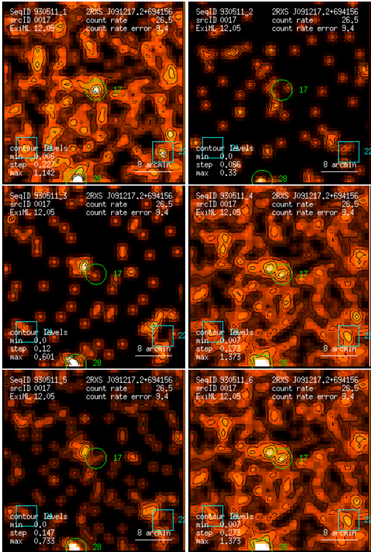
Figure 17: RASS 930511: detection 0017: band rate images, Gaussian filter: (1) PSPC channels 11 – 41, (2) 52 – 90, (3) 91 – 201, (4) 11 – 235, (5) 52 – 201, (6) 11 – 201. Broad band rates in counts/ks. Band rate contour levels in counts/ks/arcmin 2 .
