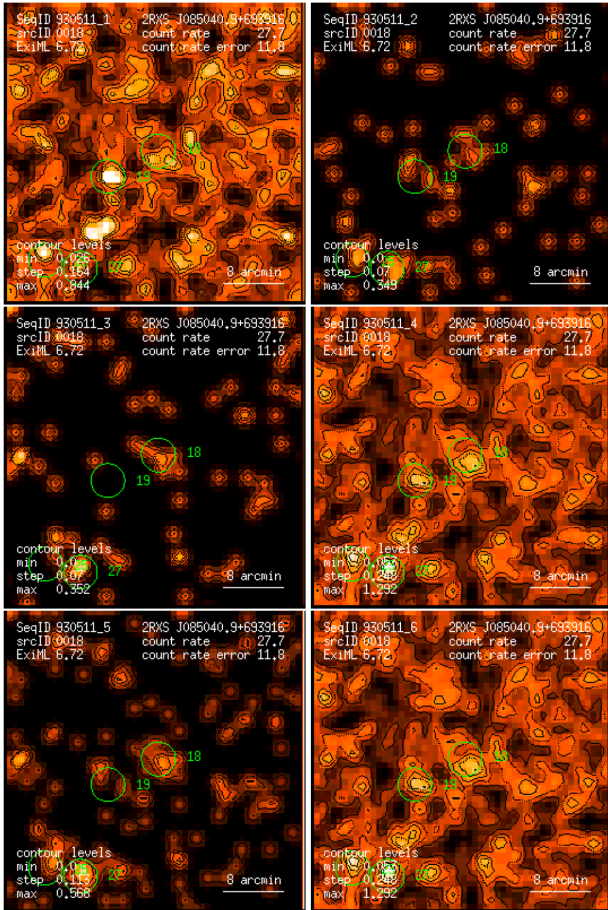
Figure 18: RASS 930511: detection 0018: band rate images, Gaussian filter: (1) PSPC channels 11 – 41, (2) 52 – 90, (3) 91 – 201, (4) 11 – 235, (5) 52 – 201, (6) 11 – 201. Broad band rates in counts/ks. Band rate contour levels in counts/ks/arcmin 2 .
