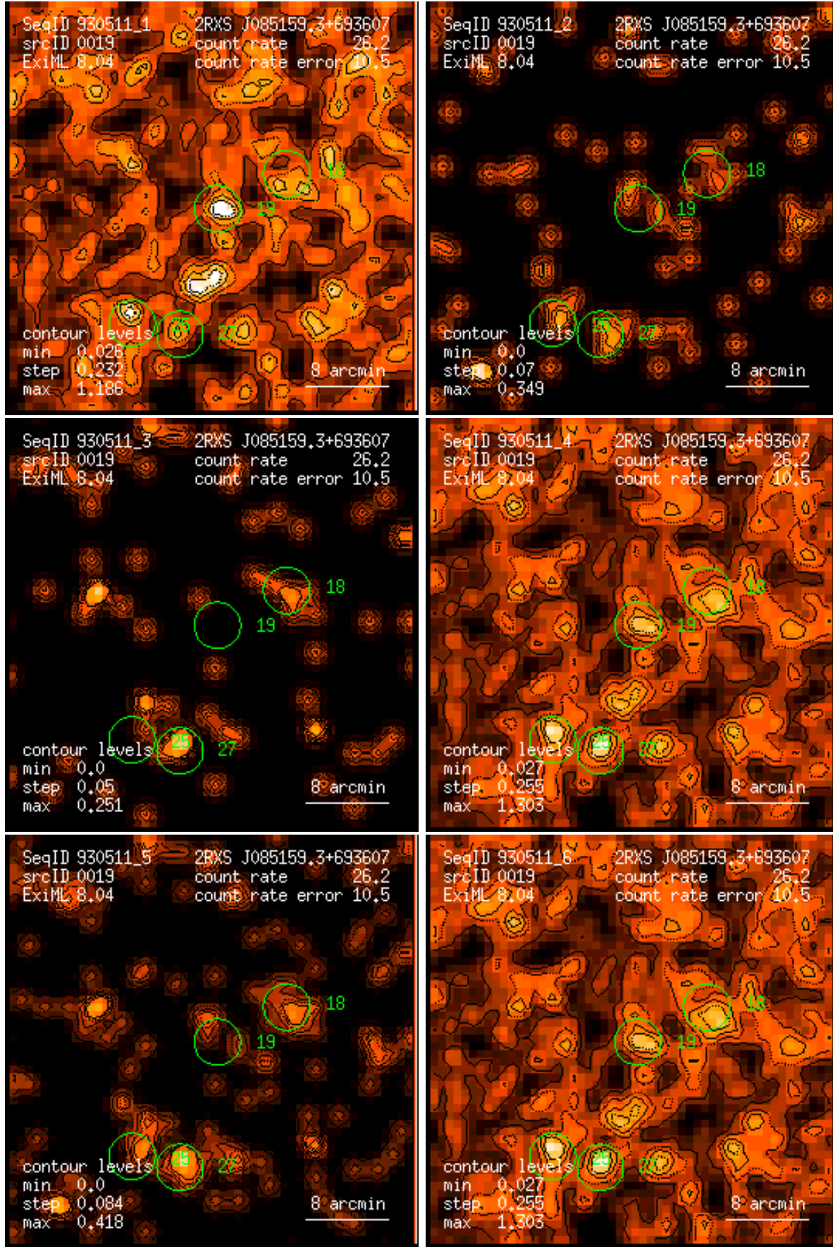
Figure 19: RASS 930511: detection 0019: band rate images, Gaussian filter: (1) PSPC channels 11 – 41, (2) 52 – 90, (3) 91 – 201, (4) 11 – 235, (5) 52 – 201, (6) 11 – 201. Broad band rates in counts/ks. Band rate contour levels in counts/ks/arcmin 2 .
