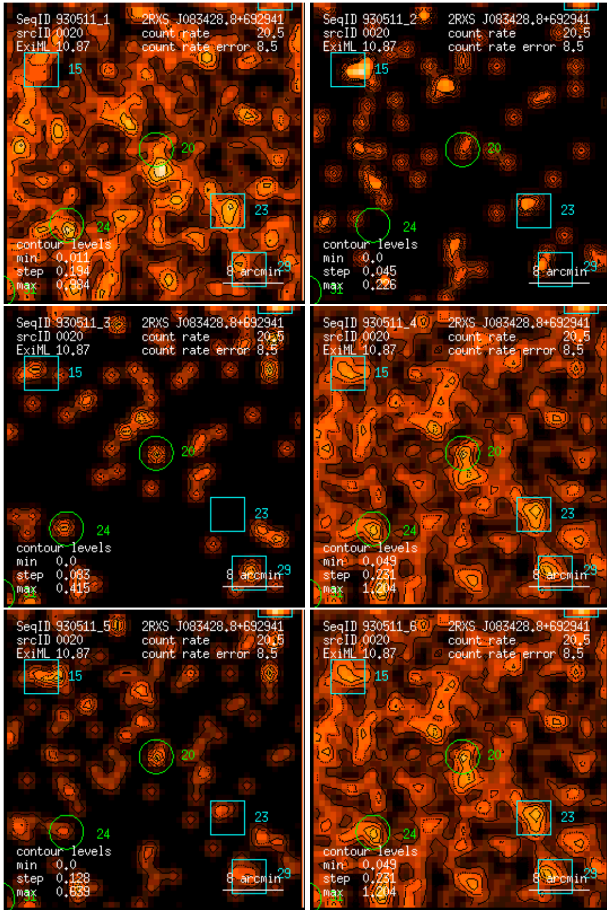
Figure 20: RASS 930511: detection 0020: band rate images, Gaussian filter: (1) PSPC channels 11 – 41, (2) 52 – 90, (3) 91 – 201, (4) 11 – 235, (5) 52 – 201, (6) 11 – 201. Broad band rates in counts/ks. Band rate contour levels in counts/ks/arcmin 2 .
