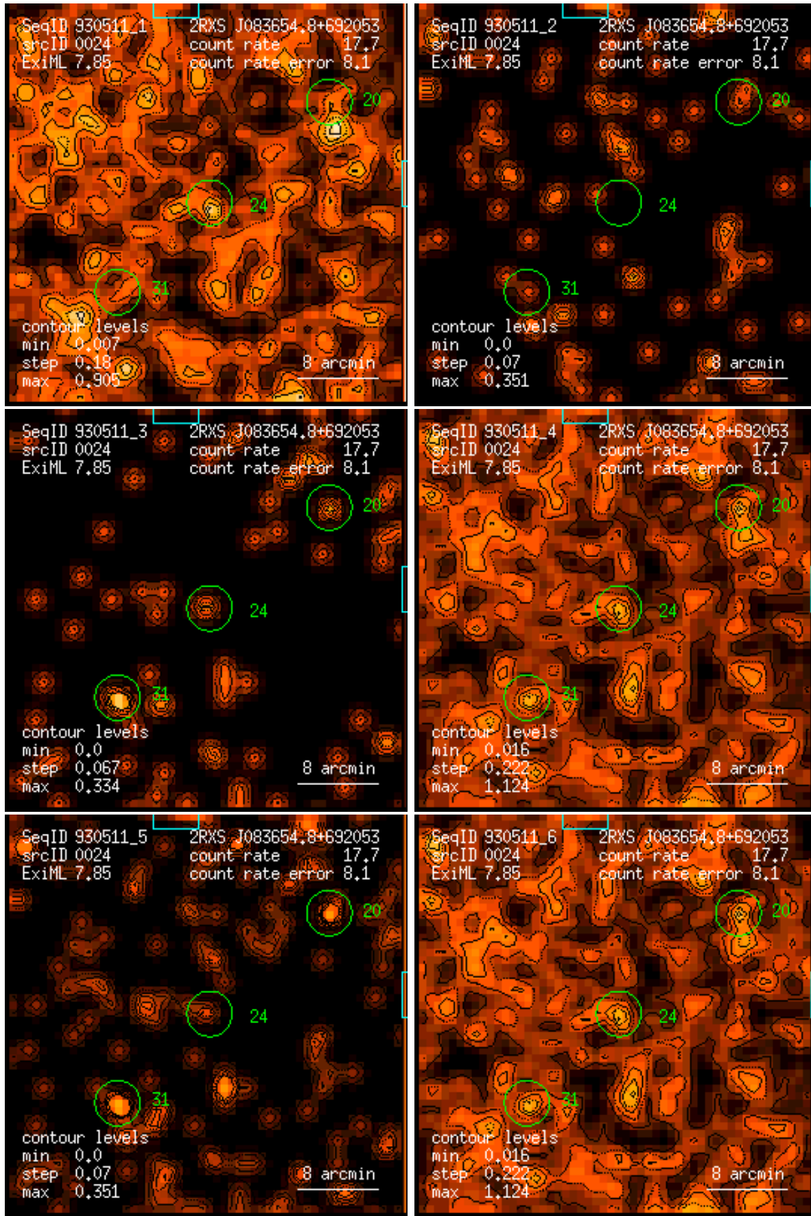
Figure 24: RASS 930511: detection 0024: band rate images, Gaussian filter: (1) PSPC channels 11 – 41, (2) 52 – 90, (3) 91 – 201, (4) 11 – 235, (5) 52 – 201, (6) 11 – 201. Broad band rates in counts/ks. Band rate contour levels in counts/ks/arcmin 2 .
