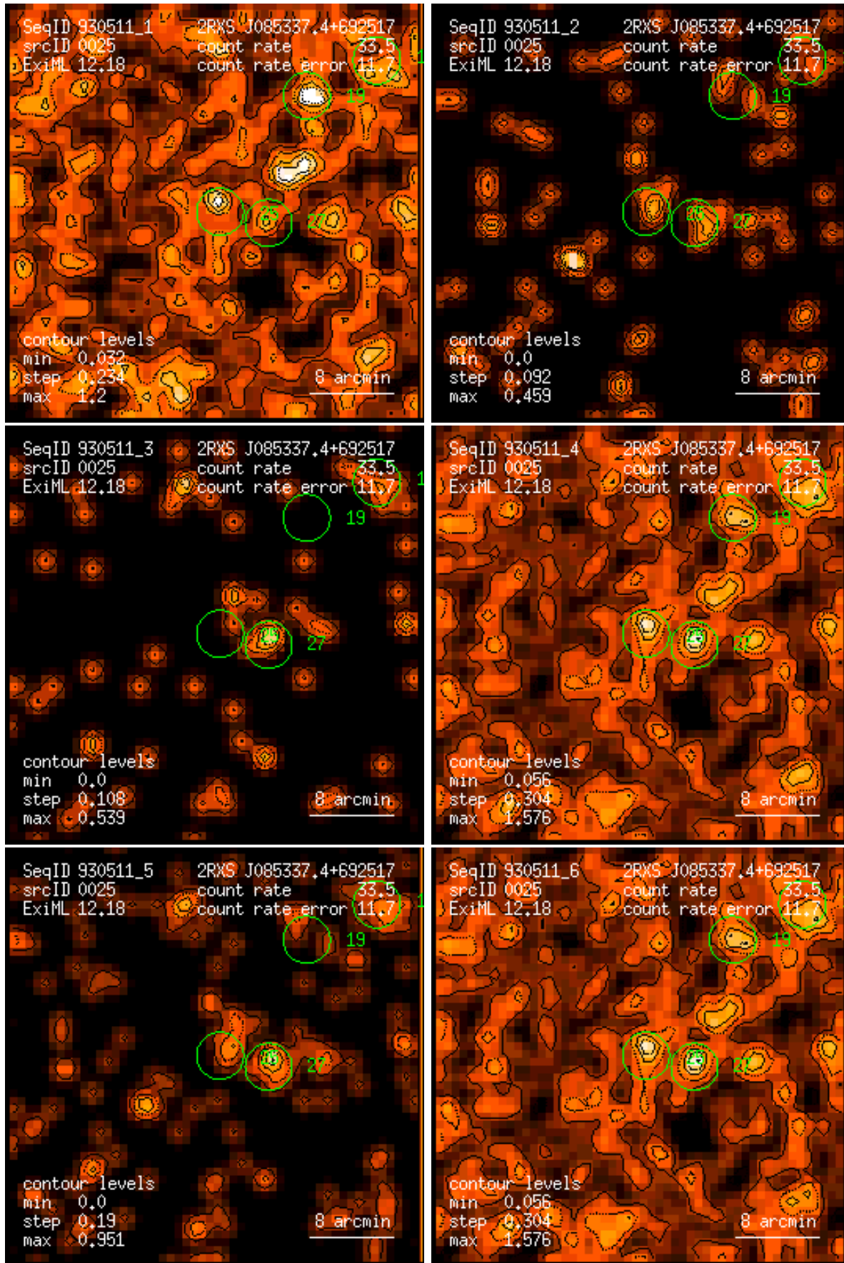
Figure 25: RASS 930511: detection 0025: band rate images, Gaussian filter: (1) PSPC channels 11 – 41, (2) 52 – 90, (3) 91 – 201, (4) 11 – 235, (5) 52 – 201, (6) 11 – 201. Broad band rates in counts/ks. Band rate contour levels in counts/ks/arcmin 2 .
