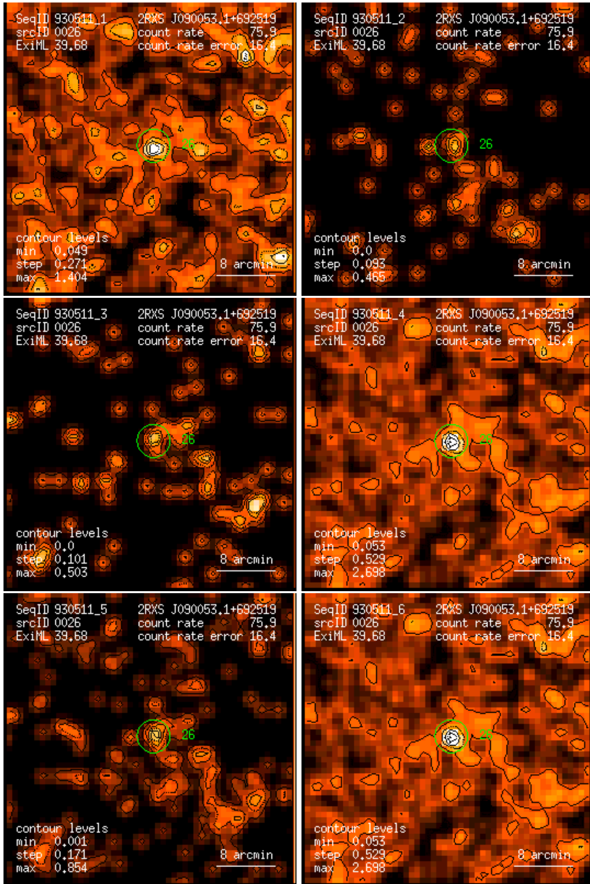
Figure 26: RASS 930511: detection 0026: band rate images, Gaussian filter: (1) PSPC channels 11 – 41, (2) 52 – 90, (3) 91 – 201, (4) 11 – 235, (5) 52 – 201, (6) 11 – 201. Broad band rates in counts/ks. Band rate contour levels in counts/ks/arcmin 2 .
