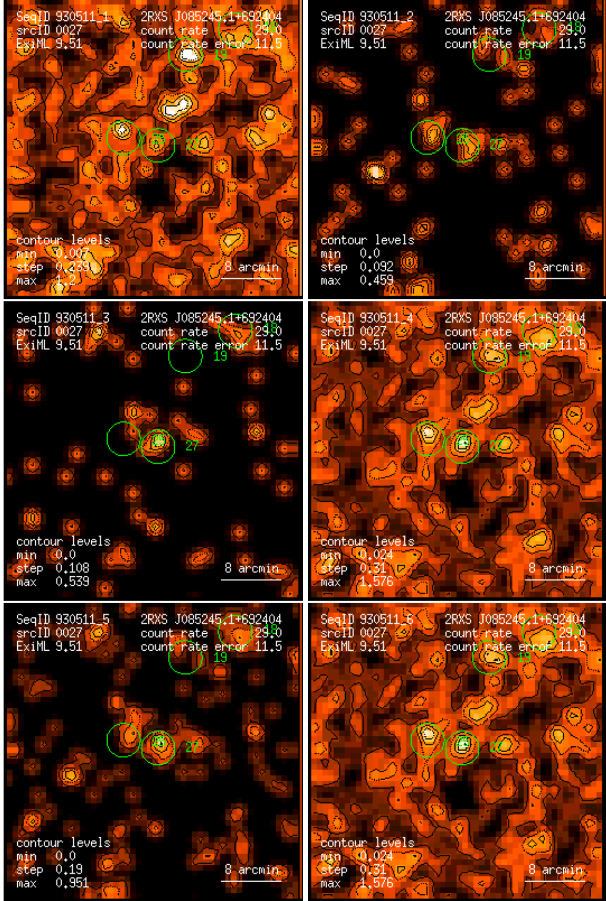
Figure 27: RASS 930511: detection 0027: band rate images, Gaussian filter: (1) PSPC channels 11 – 41, (2) 52 – 90, (3) 91 – 201, (4) 11 – 235, (5) 52 – 201, (6) 11 – 201. Broad band rates in counts/ks. Band rate contour levels in counts/ks/arcmin 2 .
