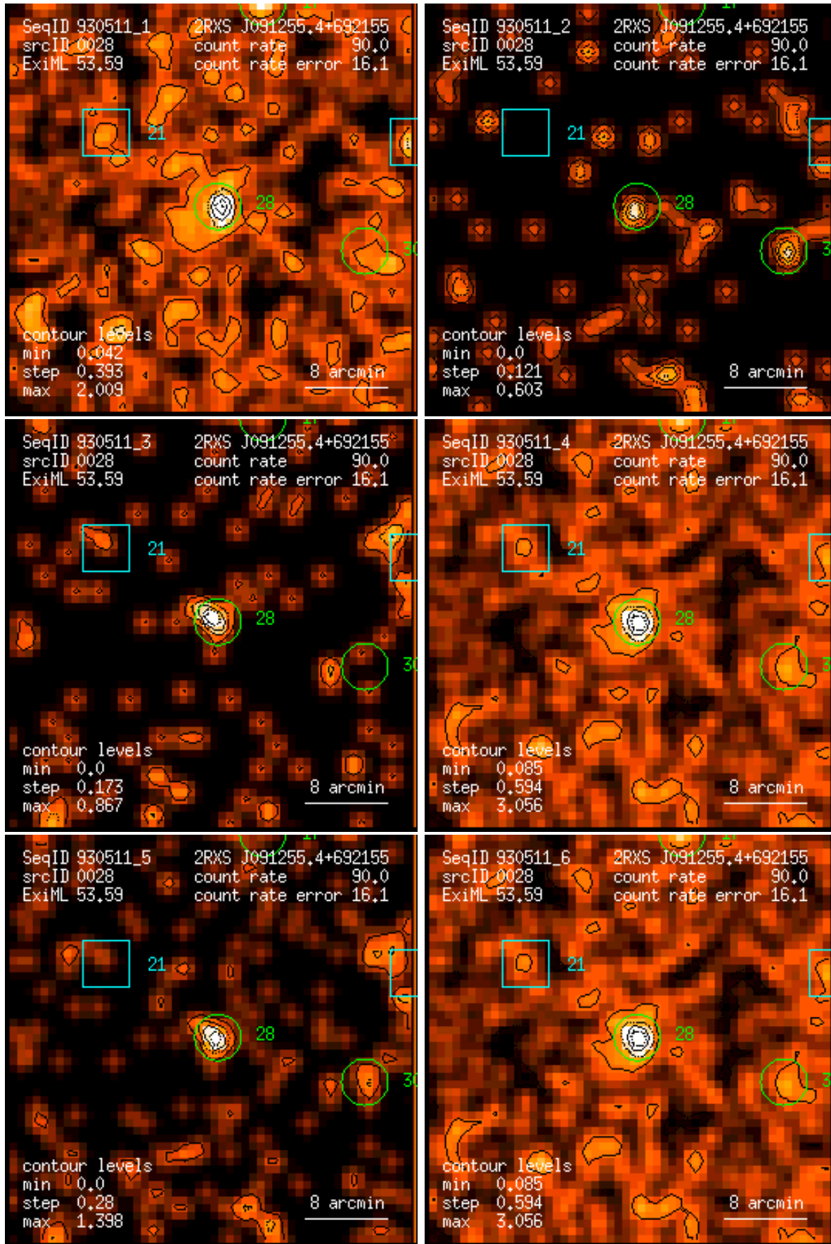
Figure 28: RASS 930511: detection 0028: band rate images, Gaussian filter: (1) PSPC channels 11 – 41, (2) 52 – 90, (3) 91 – 201, (4) 11 – 235, (5) 52 – 201, (6) 11 – 201. Broad band rates in counts/ks. Band rate contour levels in counts/ks/arcmin 2 .
