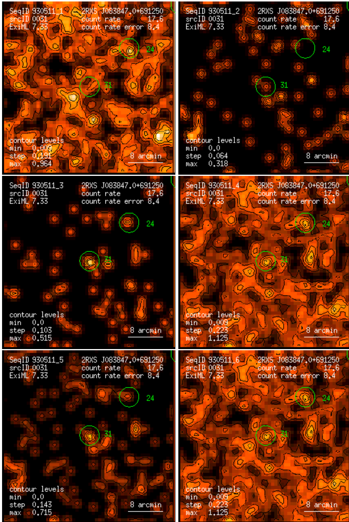
Figure 31: RASS 930511: detection 0031: band rate images, Gaussian filter: (1) PSPC channels 11 – 41, (2) 52 – 90, (3) 91 – 201, (4) 11 – 235, (5) 52 – 201, (6) 11 – 201. Broad band rates in counts/ks. Band rate contour levels in counts/ks/arcmin 2 .
