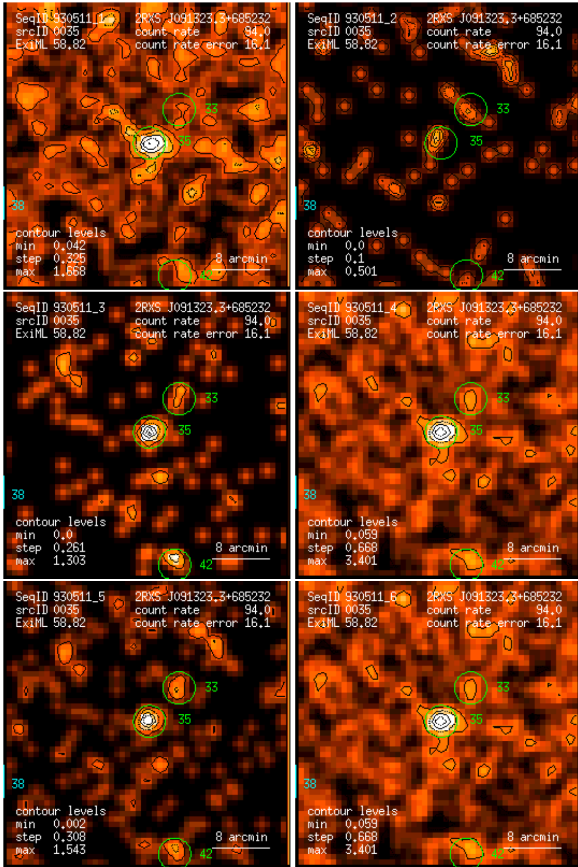
Figure 35: RASS 930511: detection 0035: band rate images, Gaussian filter: (1) PSPC channels 11 – 41, (2) 52 – 90, (3) 91 – 201, (4) 11 – 235, (5) 52 – 201, (6) 11 – 201. Broad band rates in counts/ks. Band rate contour levels in counts/ks/arcmin 2 .
