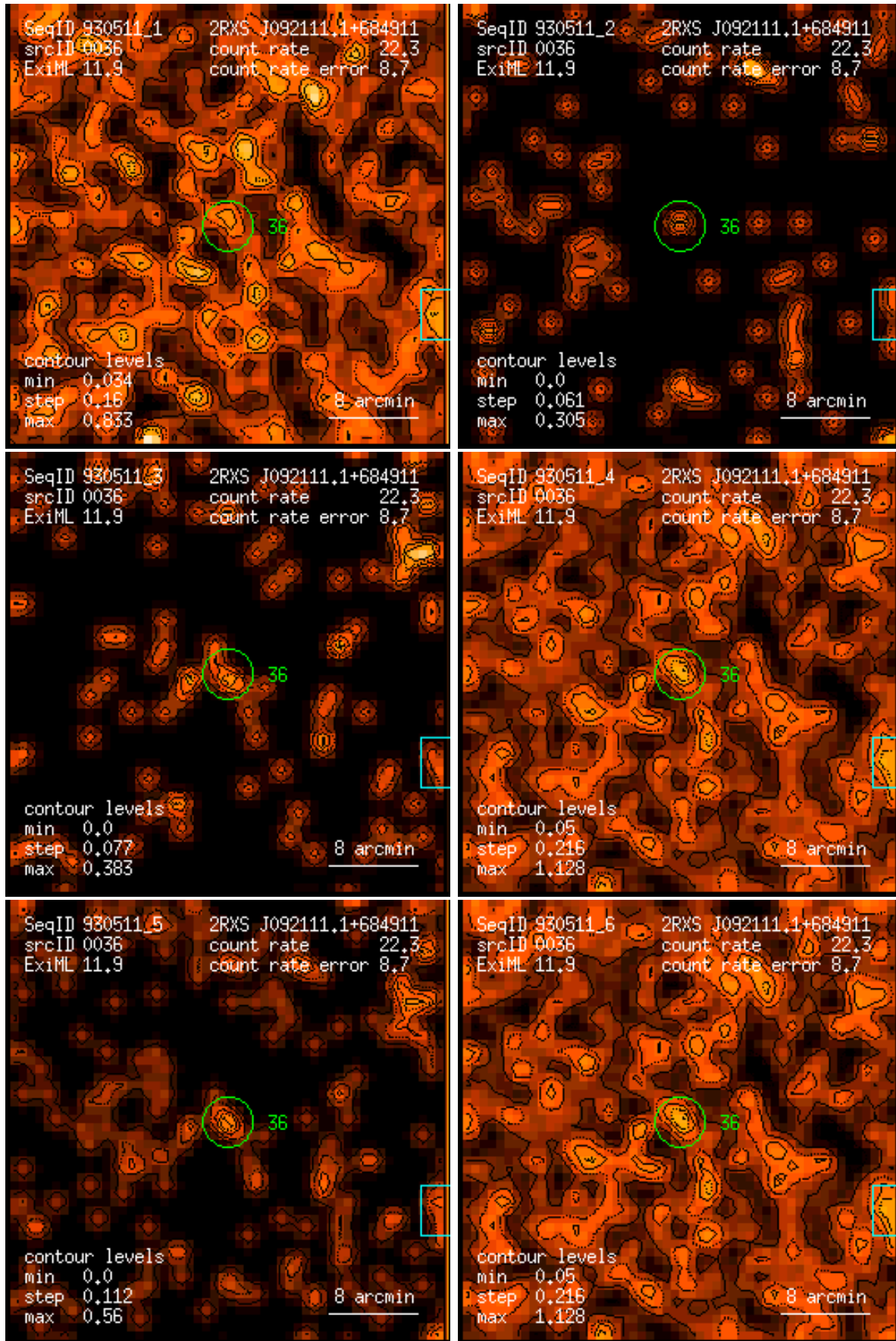
Figure 36: RASS 930511: detection 0036: band rate images, Gaussian filter: (1) PSPC channels 11 – 41, (2) 52 – 90, (3) 91 – 201, (4) 11 – 235, (5) 52 – 201, (6) 11 – 201. Broad band rates in counts/ks. Band rate contour levels in counts/ks/arcmin 2 .
