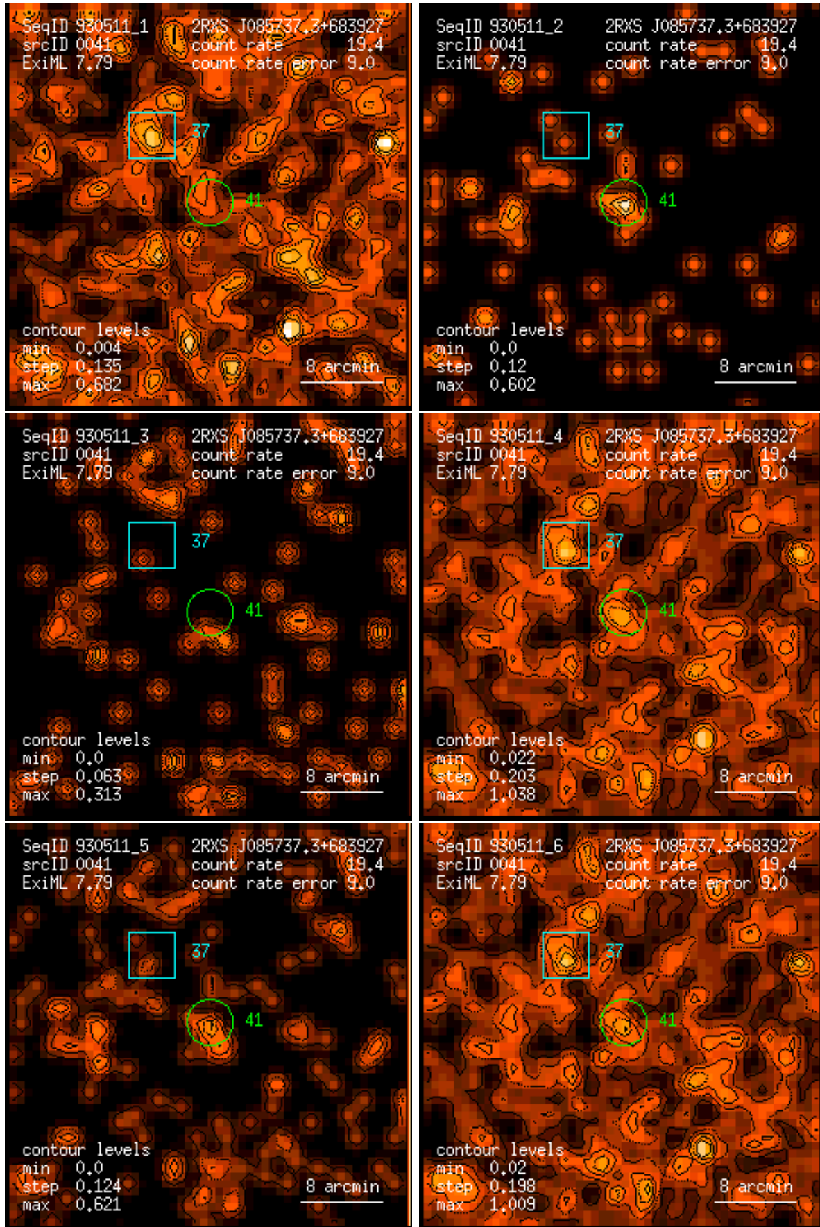
Figure 41: RASS 930511: detection 0041: band rate images, Gaussian filter: (1) PSPC channels 11 – 41, (2) 52 – 90, (3) 91 – 201, (4) 11 – 235, (5) 52 – 201, (6) 11 – 201. Broad band rates in counts/ks. Band rate contour levels in counts/ks/arcmin 2 .
