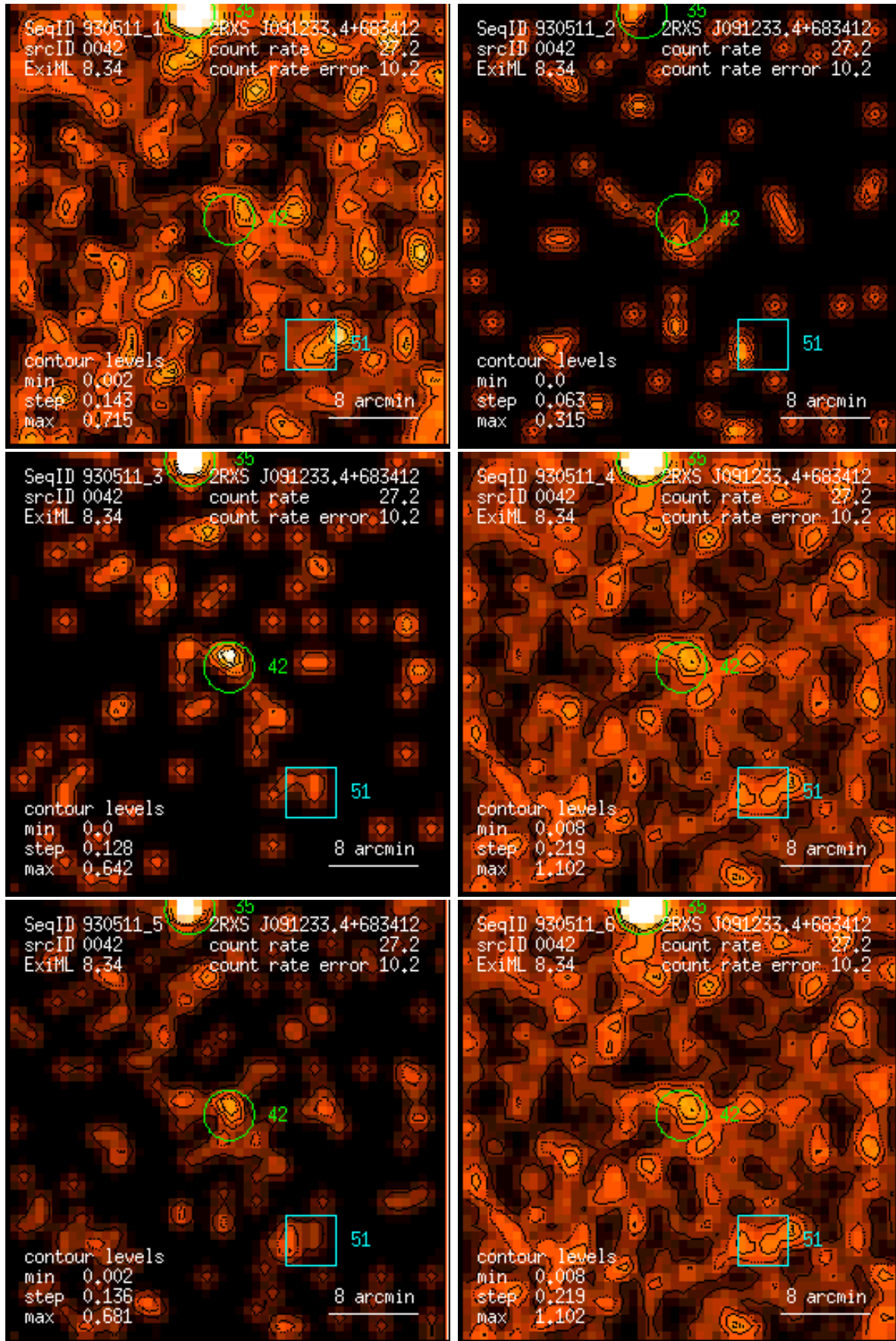
Figure 42: RASS 930511: detection 0042: band rate images, Gaussian filter: (1) PSPC channels 11 – 41, (2) 52 – 90, (3) 91 – 201, (4) 11 – 235, (5) 52 – 201, (6) 11 – 201. Broad band rates in counts/ks. Band rate contour levels in counts/ks/arcmin 2 .
