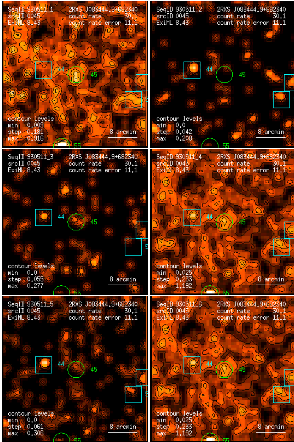
Figure 45: RASS 930511: detection 0045: band rate images, Gaussian filter: (1) PSPC channels 11 – 41, (2) 52 – 90, (3) 91 – 201, (4) 11 – 235, (5) 52 – 201, (6) 11 – 201. Broad band rates in counts/ks. Band rate contour levels in counts/ks/arcmin 2 .
