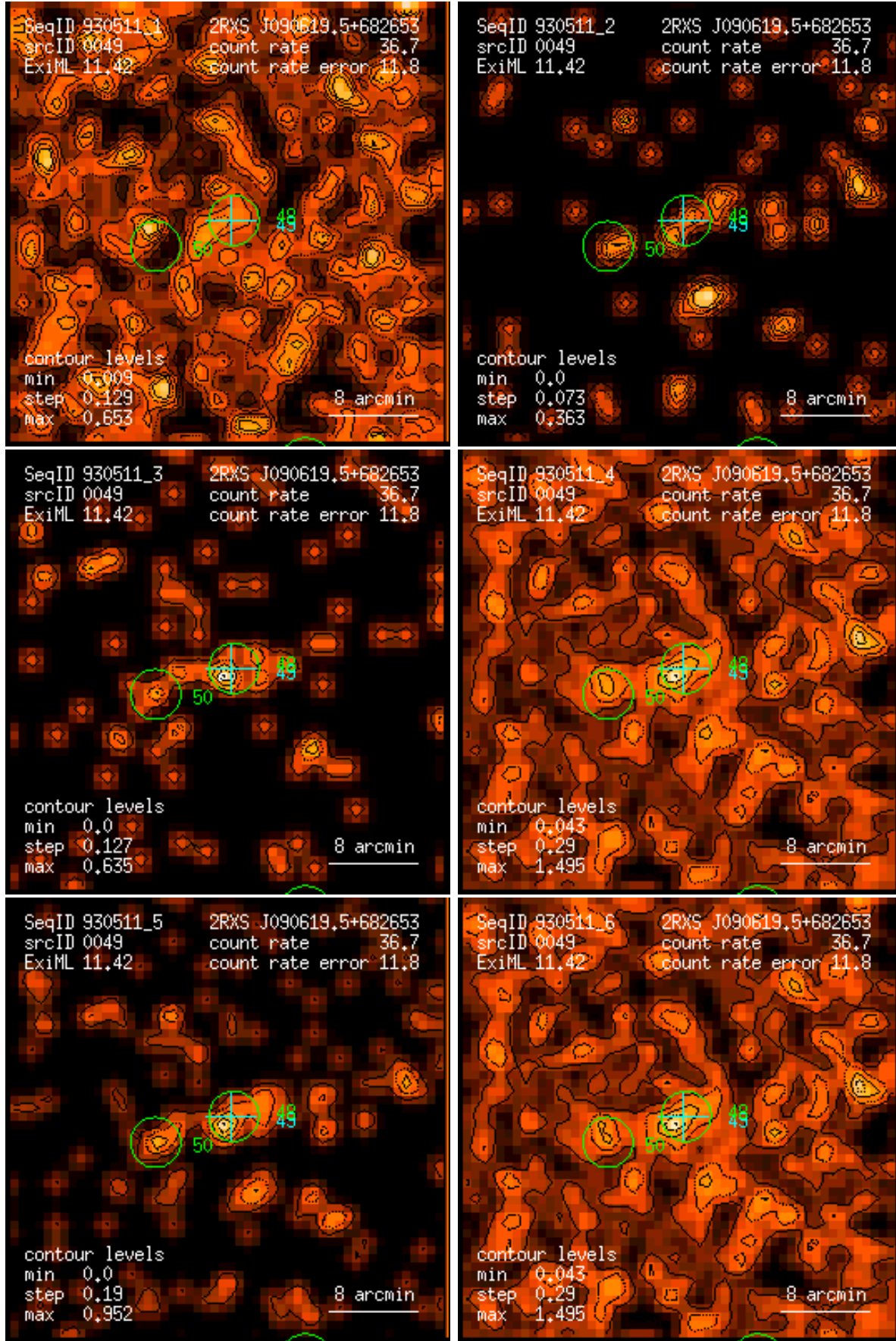
Figure 49: RASS 930511: detection 0049: band rate images, Gaussian filter: (1) PSPC channels 11 – 41, (2) 52 – 90, (3) 91 – 201, (4) 11 – 235, (5) 52 – 201, (6) 11 – 201. Broad band rates in counts/ks. Band rate contour levels in counts/ks/arcmin 2 .
