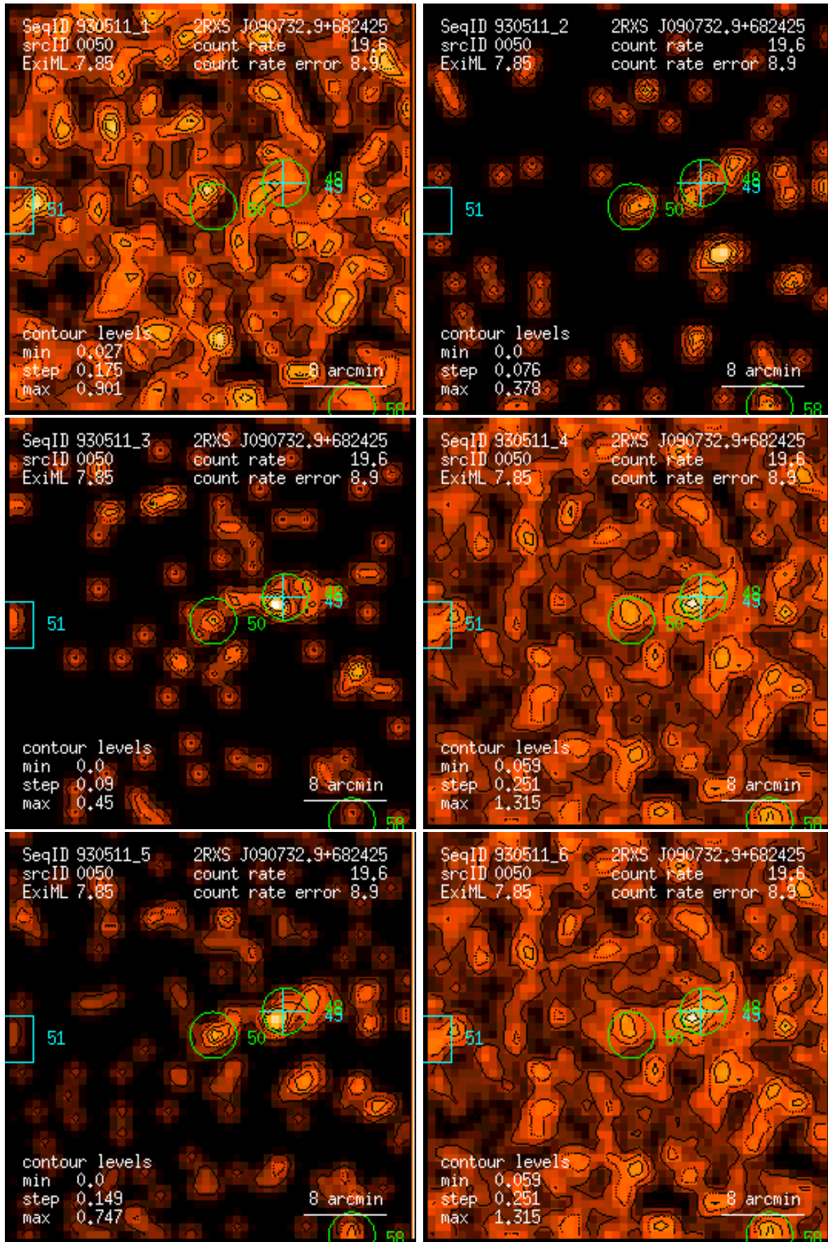
Figure 50: RASS 930511: detection 0050: band rate images, Gaussian filter: (1) PSPC channels 11 – 41, (2) 52 – 90, (3) 91 – 201, (4) 11 – 235, (5) 52 – 201, (6) 11 – 201. Broad band rates in counts/ks. Band rate contour levels in counts/ks/arcmin 2 .
