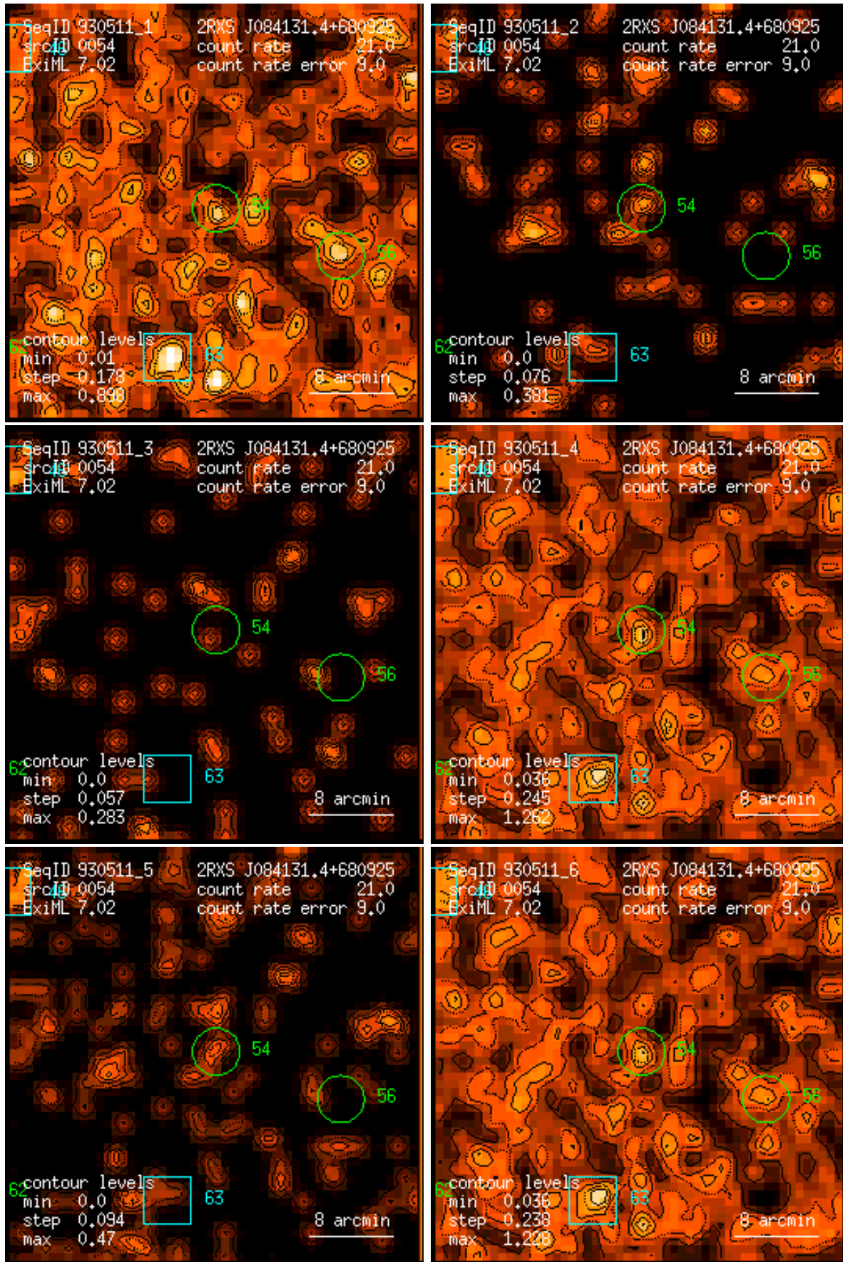
Figure 54: RASS 930511: detection 0054: band rate images, Gaussian filter: (1) PSPC channels 11 – 41, (2) 52 – 90, (3) 91 – 201, (4) 11 – 235, (5) 52 – 201, (6) 11 – 201. Broad band rates in counts/ks. Band rate contour levels in counts/ks/arcmin 2 .
