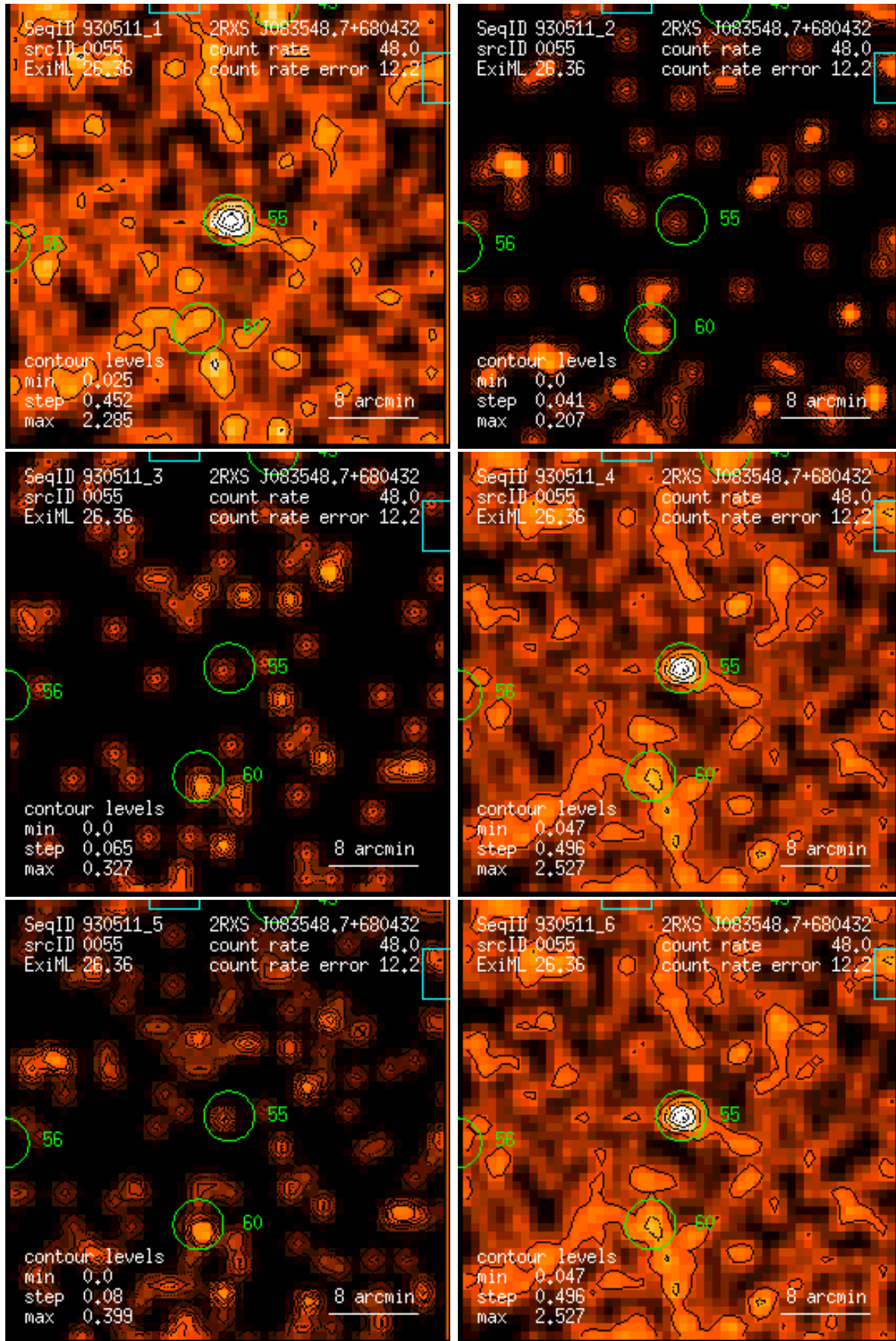
Figure 55: RASS 930511: detection 0055: band rate images, Gaussian filter: (1) PSPC channels 11 – 41, (2) 52 – 90, (3) 91 – 201, (4) 11 – 235, (5) 52 – 201, (6) 11 – 201. Broad band rates in counts/ks. Band rate contour levels in counts/ks/arcmin 2 .
