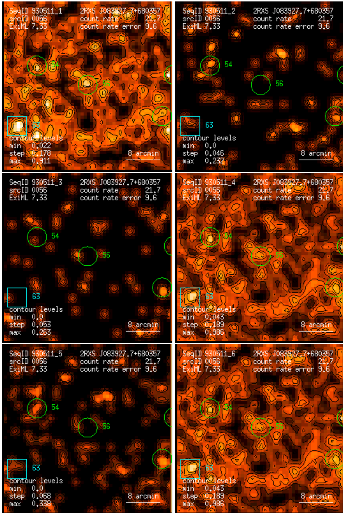
Figure 56: RASS 930511: detection 0056: band rate images, Gaussian filter: (1) PSPC channels 11 – 41, (2) 52 – 90, (3) 91 – 201, (4) 11 – 235, (5) 52 – 201, (6) 11 – 201. Broad band rates in counts/ks. Band rate contour levels in counts/ks/arcmin 2 .
