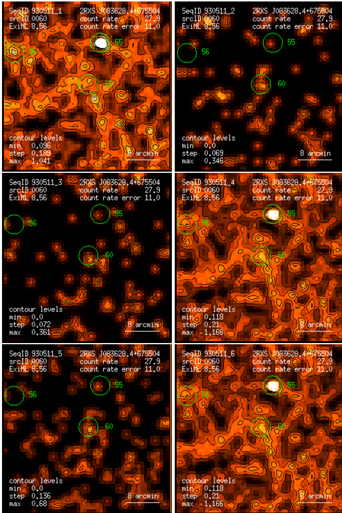
Figure 60: RASS 930511: detection 0060: band rate images, Gaussian filter: (1) PSPC channels 11 – 41, (2) 52 – 90, (3) 91 – 201, (4) 11 – 235, (5) 52 – 201, (6) 11 – 201. Broad band rates in counts/ks. Band rate contour levels in counts/ks/arcmin 2 .
