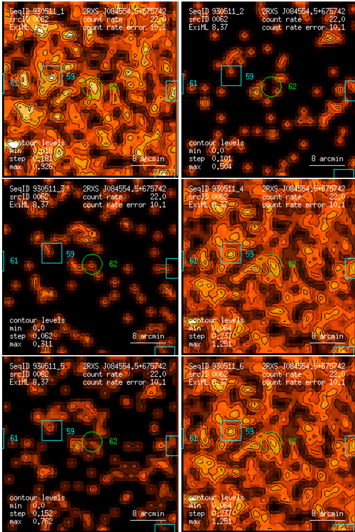
Figure 62: RASS 930511: detection 0062: band rate images, Gaussian filter: (1) PSPC channels 11 – 41, (2) 52 – 90, (3) 91 – 201, (4) 11 – 235, (5) 52 – 201, (6) 11 – 201. Broad band rates in counts/ks. Band rate contour levels in counts/ks/arcmin 2 .
