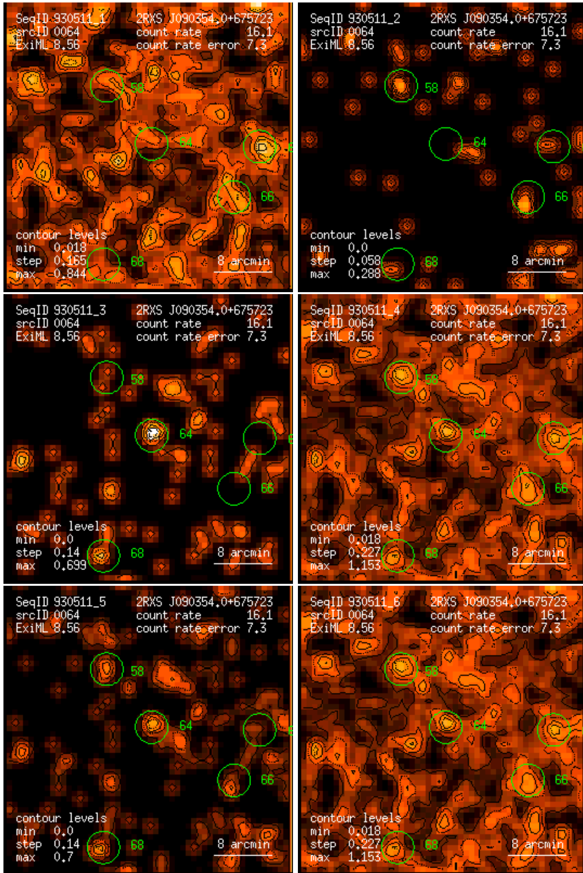
Figure 64: RASS 930511: detection 0064: band rate images, Gaussian filter: (1) PSPC channels 11 – 41, (2) 52 – 90, (3) 91 – 201, (4) 11 – 235, (5) 52 – 201, (6) 11 – 201. Broad band rates in counts/ks. Band rate contour levels in counts/ks/arcmin 2 .
