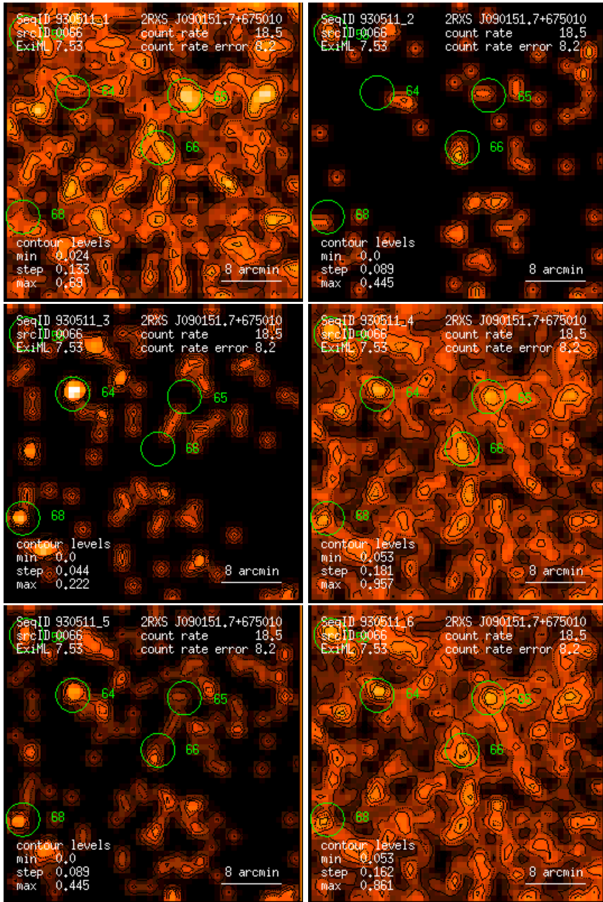
Figure 66: RASS 930511: detection 0066: band rate images, Gaussian filter: (1) PSPC channels 11 – 41, (2) 52 – 90, (3) 91 – 201, (4) 11 – 235, (5) 52 – 201, (6) 11 – 201. Broad band rates in counts/ks. Band rate contour levels in counts/ks/arcmin 2 .
