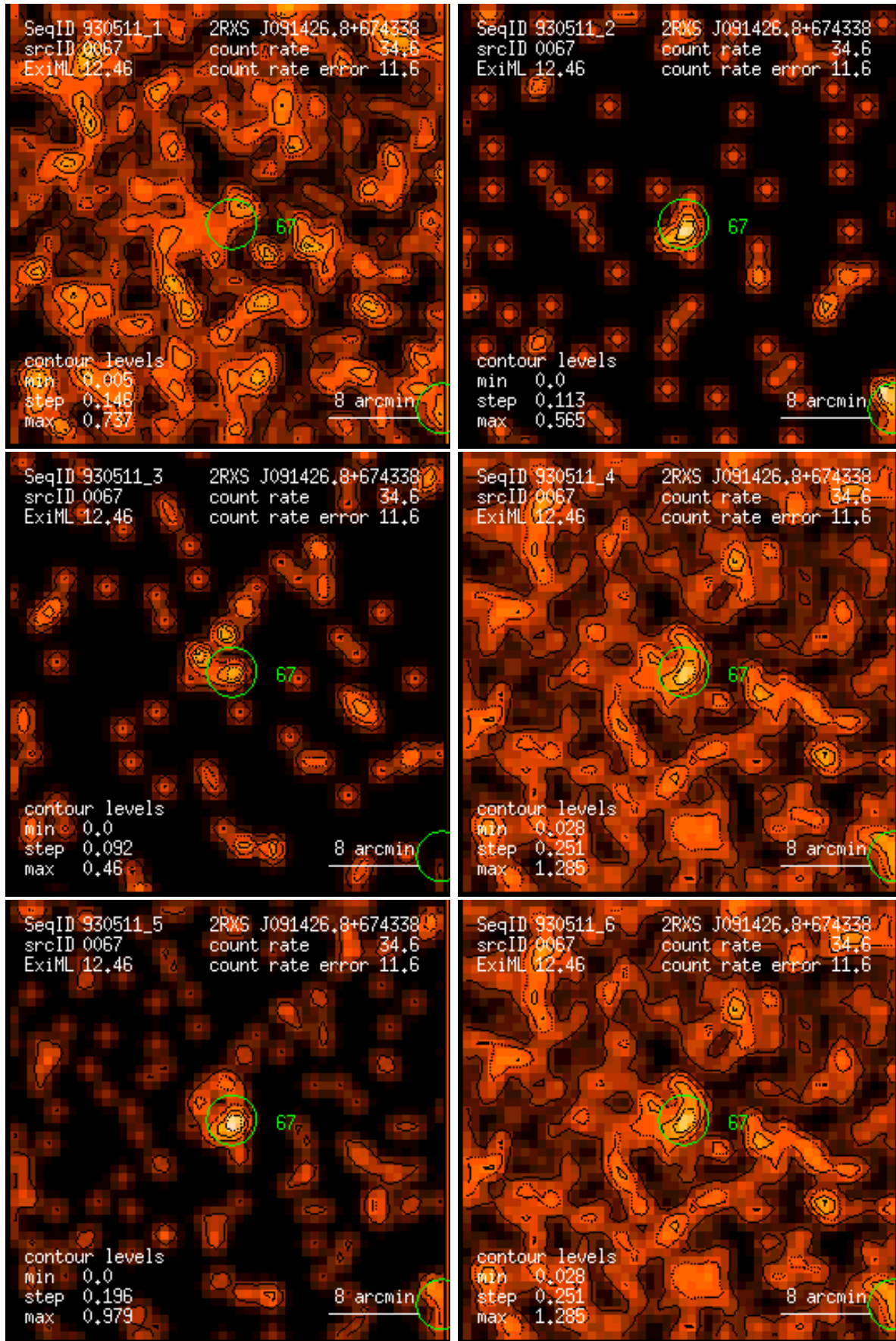
Figure 67: RASS 930511: detection 0067: band rate images, Gaussian filter: (1) PSPC channels 11 – 41, (2) 52 – 90, (3) 91 – 201, (4) 11 – 235, (5) 52 – 201, (6) 11 – 201. Broad band rates in counts/ks. Band rate contour levels in counts/ks/arcmin 2 .
