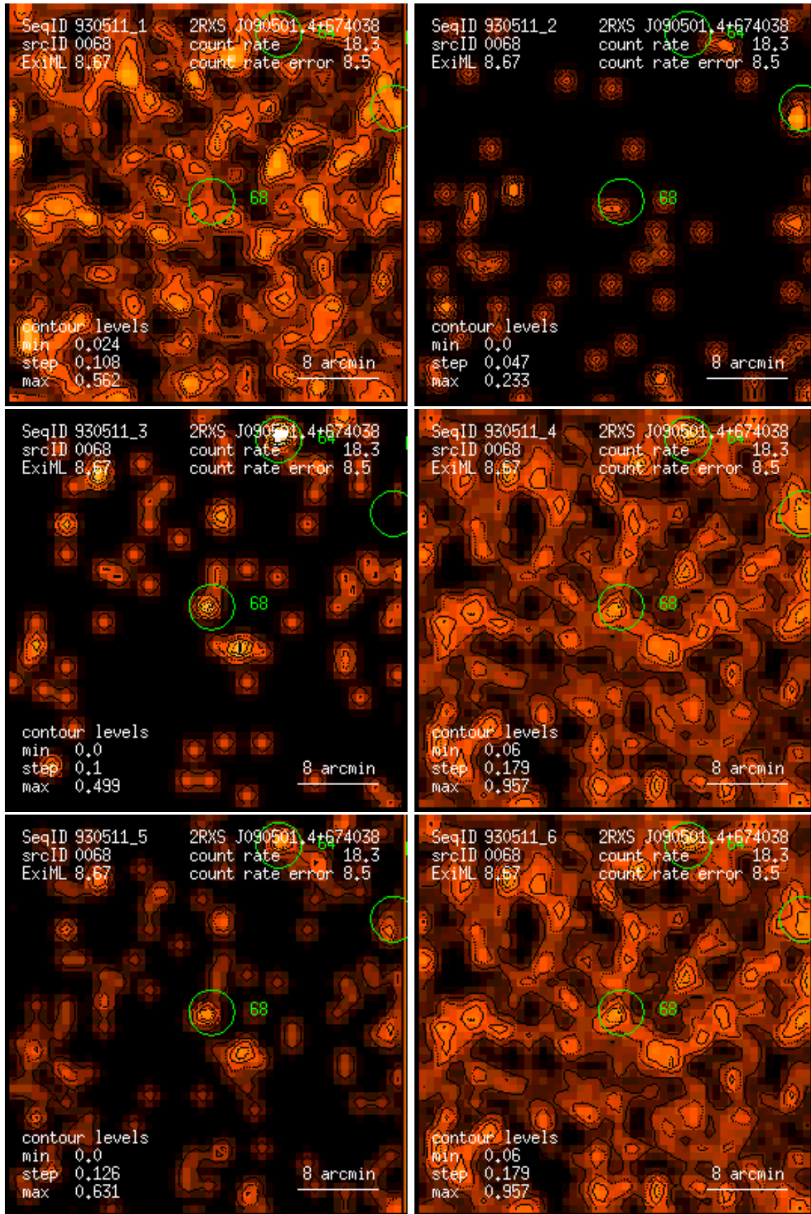
Figure 68: RASS 930511: detection 0068: band rate images, Gaussian filter: (1) PSPC channels 11 – 41, (2) 52 – 90, (3) 91 – 201, (4) 11 – 235, (5) 52 – 201, (6) 11 – 201. Broad band rates in counts/ks. Band rate contour levels in counts/ks/arcmin 2 .
