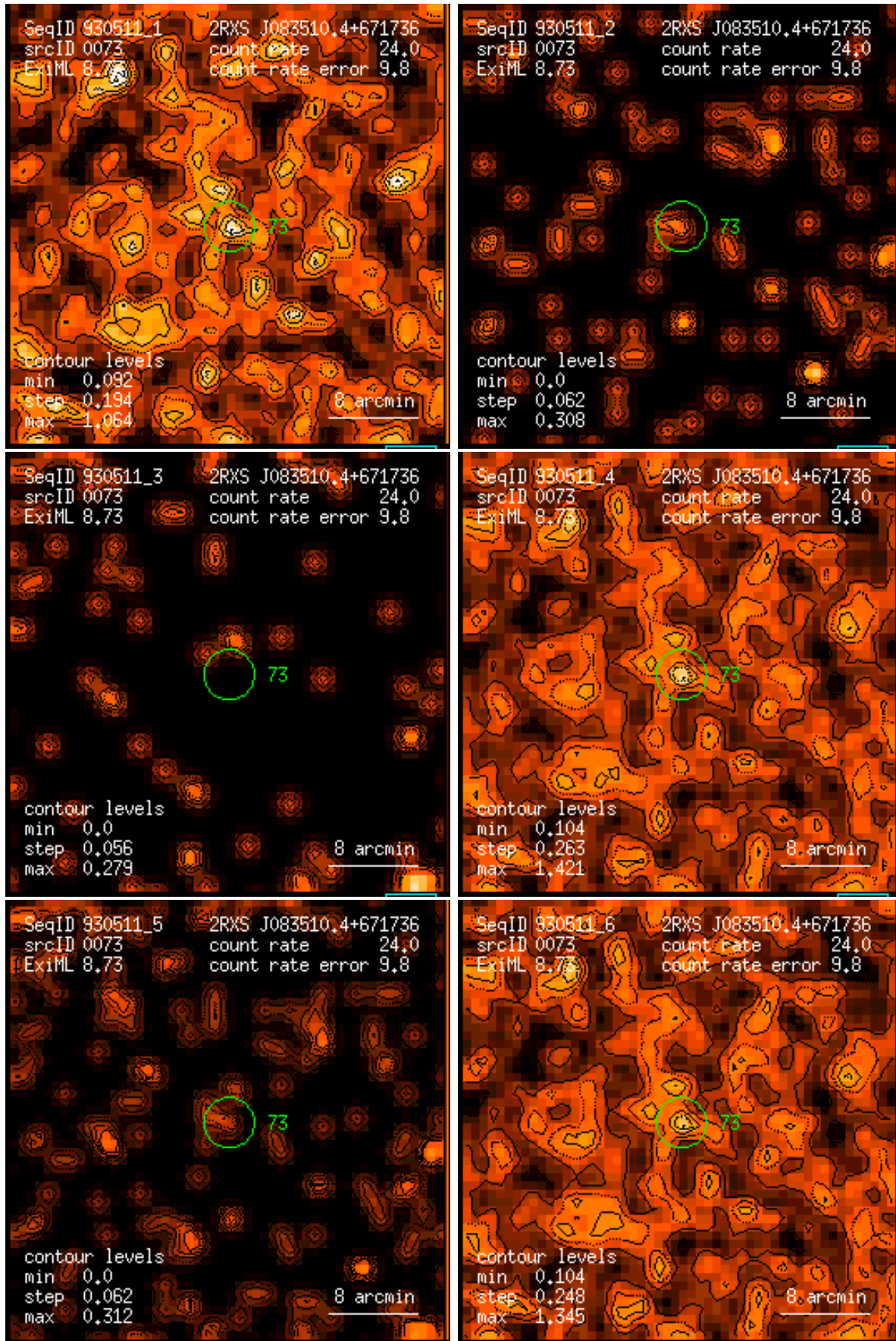
Figure 73: RASS 930511: detection 0073: band rate images, Gaussian filter: (1) PSPC channels 11 – 41, (2) 52 – 90, (3) 91 – 201, (4) 11 – 235, (5) 52 – 201, (6) 11 – 201. Broad band rates in counts/ks. Band rate contour levels in counts/ks/arcmin 2 .
