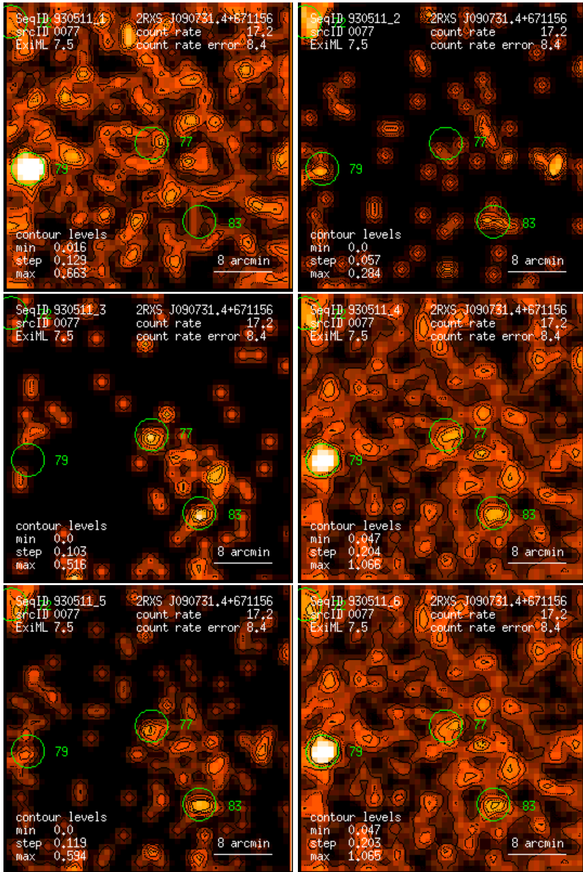
Figure 77: RASS 930511: detection 0077: band rate images, Gaussian filter: (1) PSPC channels 11 – 41, (2) 52 – 90, (3) 91 – 201, (4) 11 – 235, (5) 52 – 201, (6) 11 – 201. Broad band rates in counts/ks. Band rate contour levels in counts/ks/arcmin 2 .
