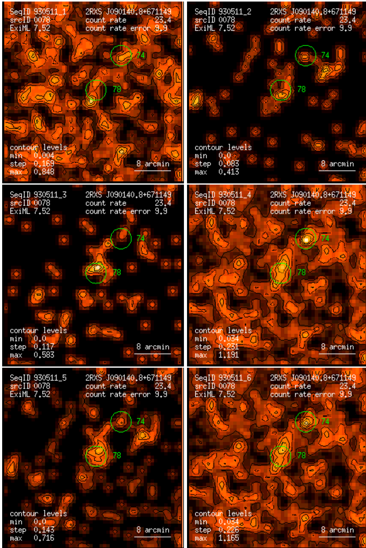
Figure 78: RASS 930511: detection 0078: band rate images, Gaussian filter: (1) PSPC channels 11 – 41, (2) 52 – 90, (3) 91 – 201, (4) 11 – 235, (5) 52 – 201, (6) 11 – 201. Broad band rates in counts/ks. Band rate contour levels in counts/ks/arcmin 2 .
