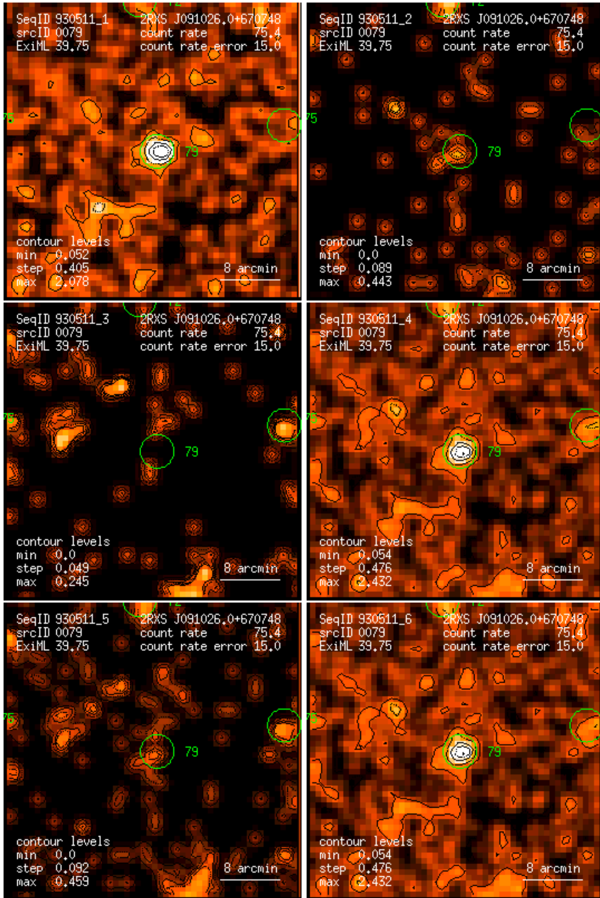
Figure 79: RASS 930511: detection 0079: band rate images, Gaussian filter: (1) PSPC channels 11 – 41, (2) 52 – 90, (3) 91 – 201, (4) 11 – 235, (5) 52 – 201, (6) 11 – 201. Broad band rates in counts/ks. Band rate contour levels in counts/ks/arcmin 2 .
