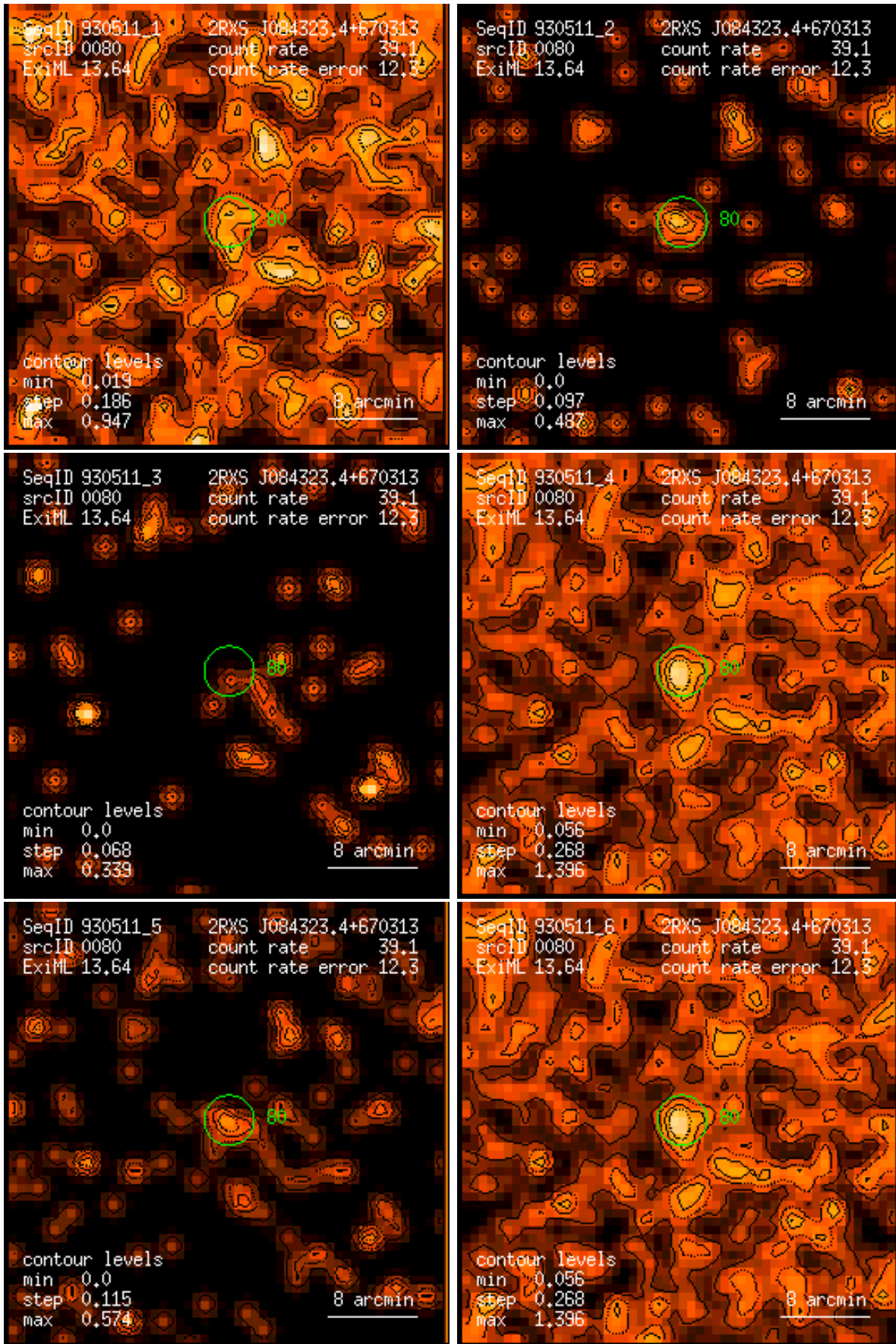
Figure 80: RASS 930511: detection 0080: band rate images, Gaussian filter: (1) PSPC channels 11 – 41, (2) 52 – 90, (3) 91 – 201, (4) 11 – 235, (5) 52 – 201, (6) 11 – 201. Broad band rates in counts/ks. Band rate contour levels in counts/ks/arcmin 2 .
